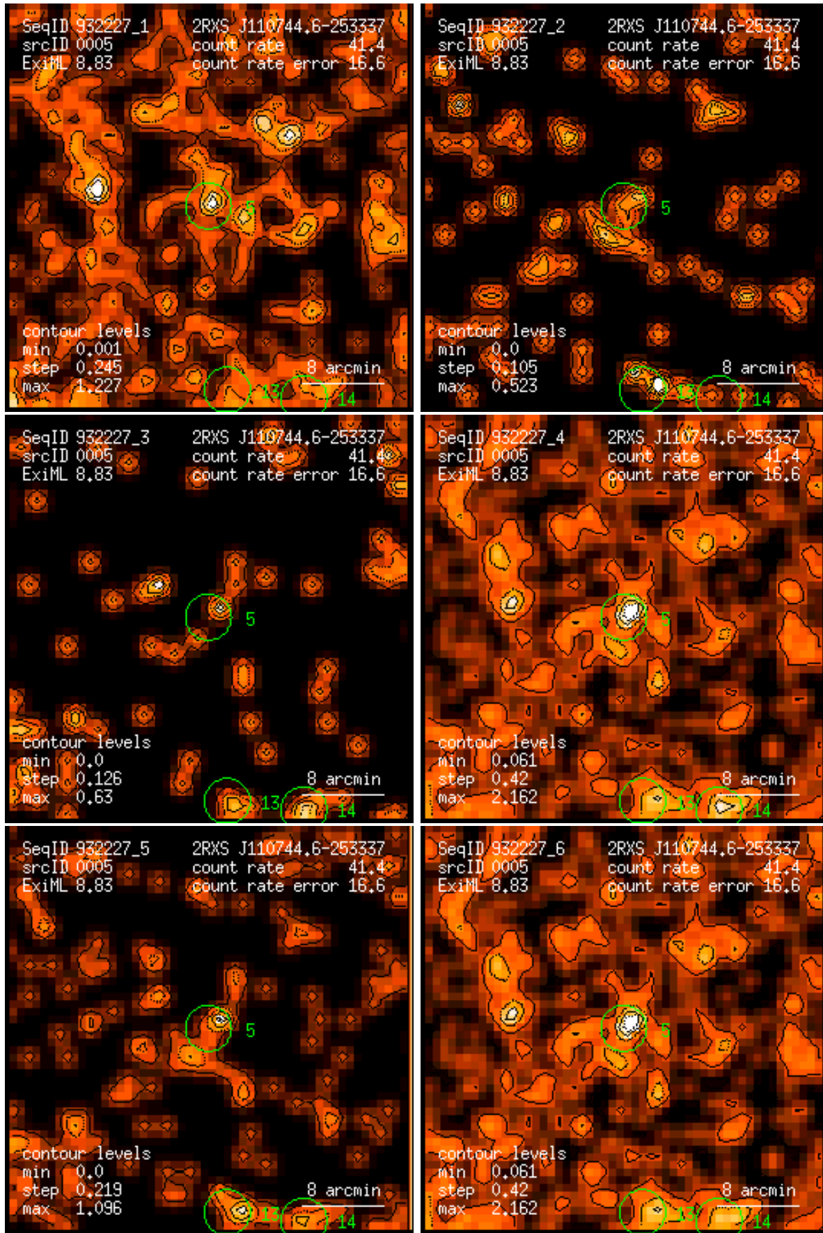
Figure 5: RASS 932227: detection 0005: band rate images, Gaussian filter: (1) PSPC channels 11 – 41, (2) 52 – 90, (3) 91 – 201, (4) 11 – 235, (5) 52 – 201, (6) 11 – 201. Broad band rates in counts/ks. Band rate contour levels in counts/ks/arcmin 2 .
