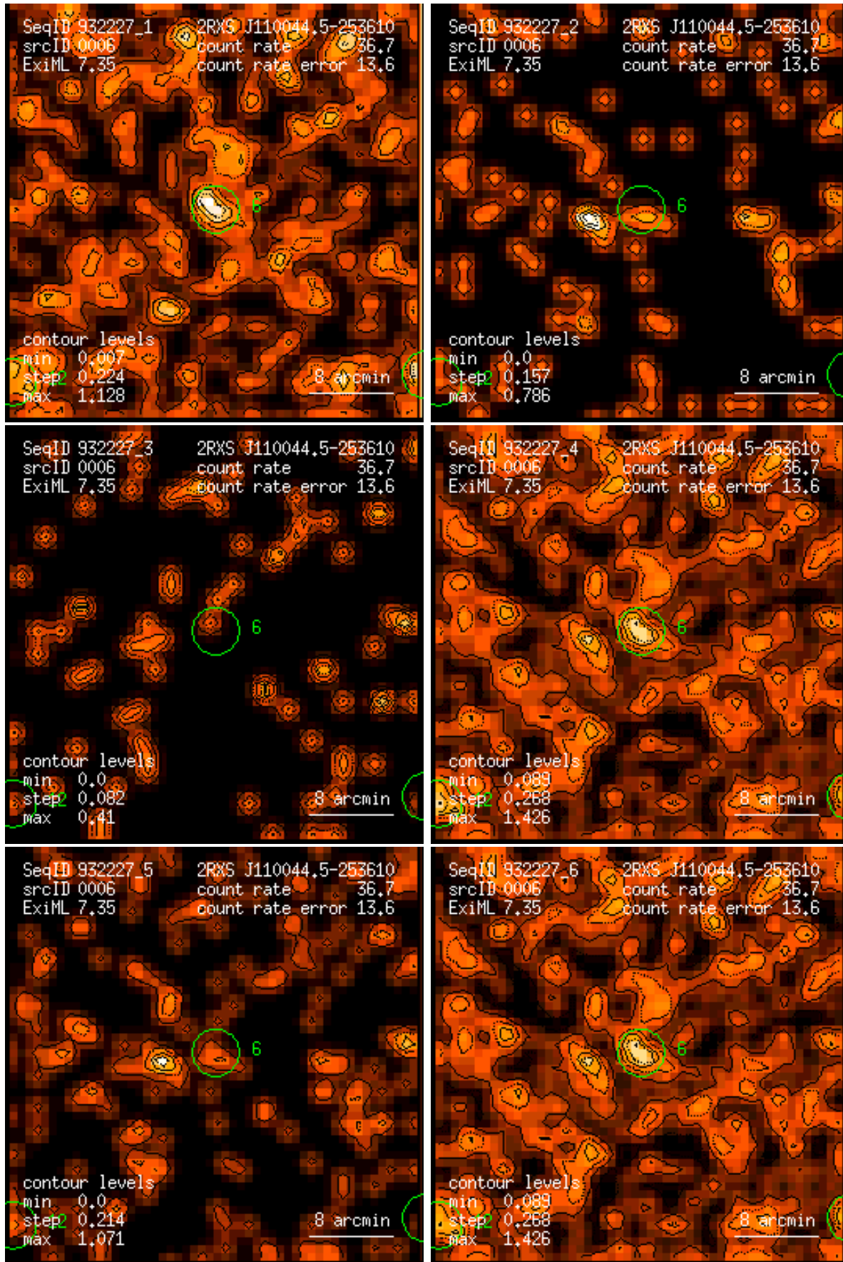
Figure 6: RASS 932227: detection 0006: band rate images, Gaussian filter: (1) PSPC channels 11 – 41, (2) 52 – 90, (3) 91 – 201, (4) 11 – 235, (5) 52 – 201, (6) 11 – 201. Broad band rates in counts/ks. Band rate contour levels in counts/ks/arcmin 2 .
