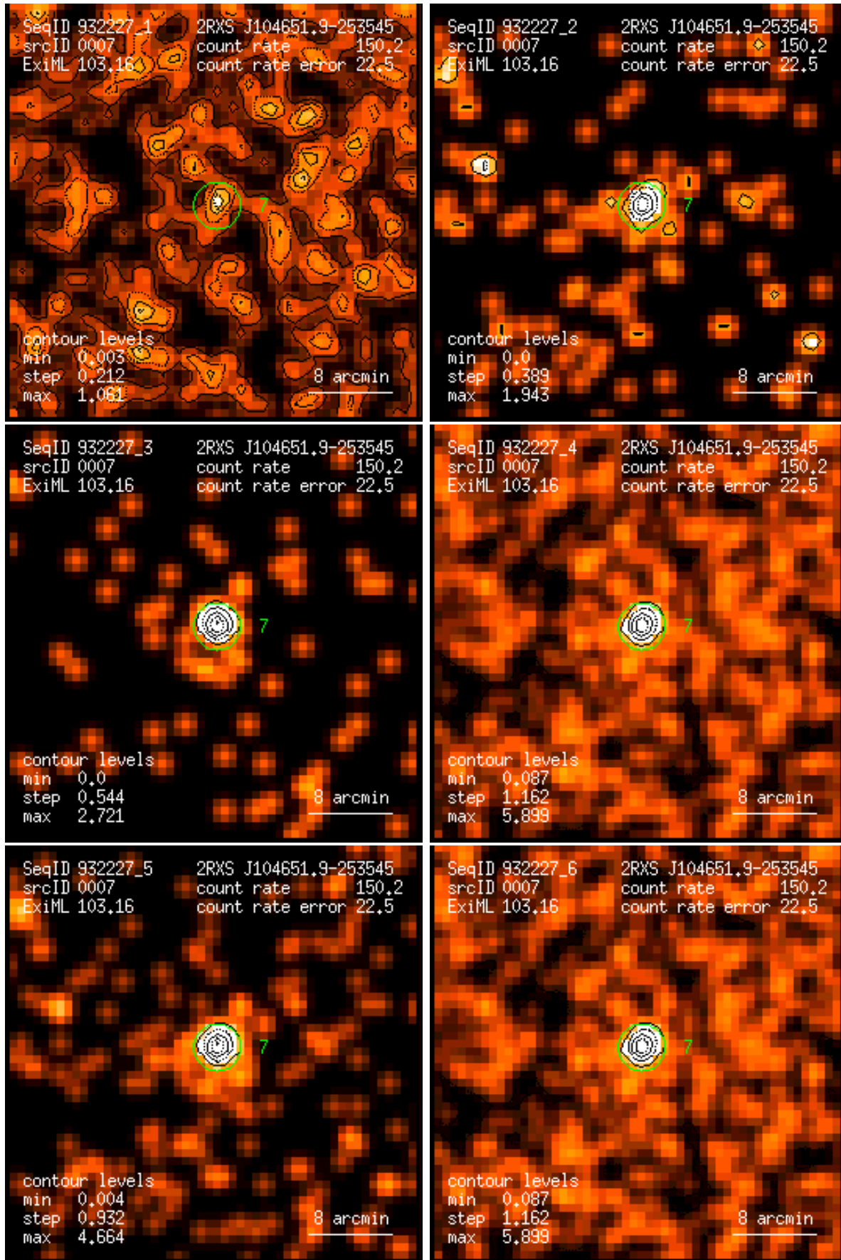
Figure 7: RASS 932227: detection 0007: band rate images, Gaussian filter: (1) PSPC channels 11 – 41, (2) 52 – 90, (3) 91 – 201, (4) 11 – 235, (5) 52 – 201, (6) 11 – 201. Broad band rates in counts/ks. Band rate contour levels in counts/ks/arcmin 2 .
