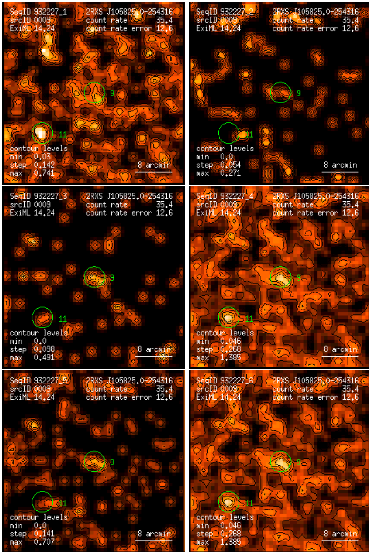
Figure 9: RASS 932227: detection 0009: band rate images, Gaussian filter: (1) PSPC channels 11 – 41, (2) 52 – 90, (3) 91 – 201, (4) 11 – 235, (5) 52 – 201, (6) 11 – 201. Broad band rates in counts/ks. Band rate contour levels in counts/ks/arcmin 2 .
