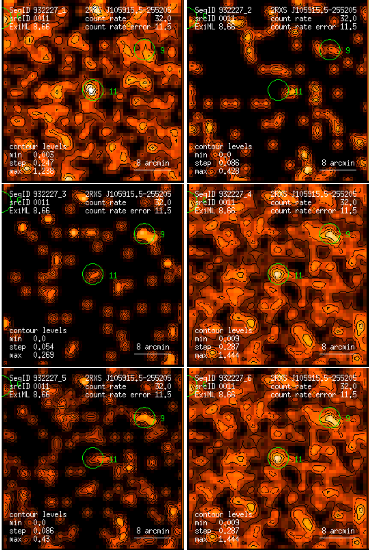
Figure 11: RASS 932227: detection 0011: band rate images, Gaussian filter: (1) PSPC channels 11 – 41, (2) 52 – 90, (3) 91 – 201, (4) 11 – 235, (5) 52 – 201, (6) 11 – 201. Broad band rates in counts/ks. Band rate contour levels in counts/ks/arcmin 2 .
