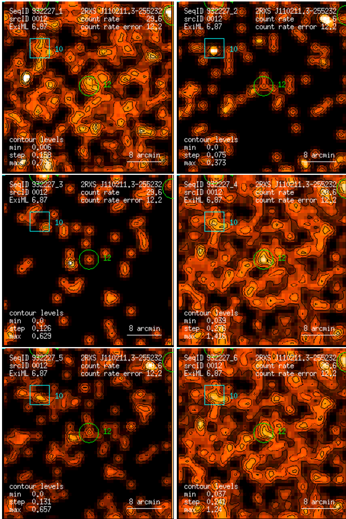
Figure 12: RASS 932227: detection 0012: band rate images, Gaussian filter: (1) PSPC channels 11 – 41, (2) 52 – 90, (3) 91 – 201, (4) 11 – 235, (5) 52 – 201, (6) 11 – 201. Broad band rates in counts/ks. Band rate contour levels in counts/ks/arcmin 2 .
