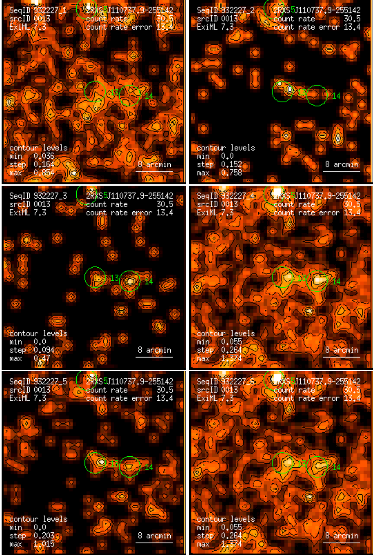
Figure 13: RASS 932227: detection 0013: band rate images, Gaussian filter: (1) PSPC channels 11 – 41, (2) 52 – 90, (3) 91 – 201, (4) 11 – 235, (5) 52 – 201, (6) 11 – 201. Broad band rates in counts/ks. Band rate contour levels in counts/ks/arcmin 2 .
