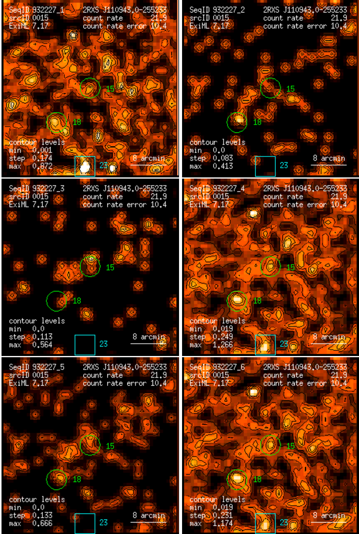
Figure 15: RASS 932227: detection 0015: band rate images, Gaussian filter: (1) PSPC channels 11 – 41, (2) 52 – 90, (3) 91 – 201, (4) 11 – 235, (5) 52 – 201, (6) 11 – 201. Broad band rates in counts/ks. Band rate contour levels in counts/ks/arcmin 2 .
