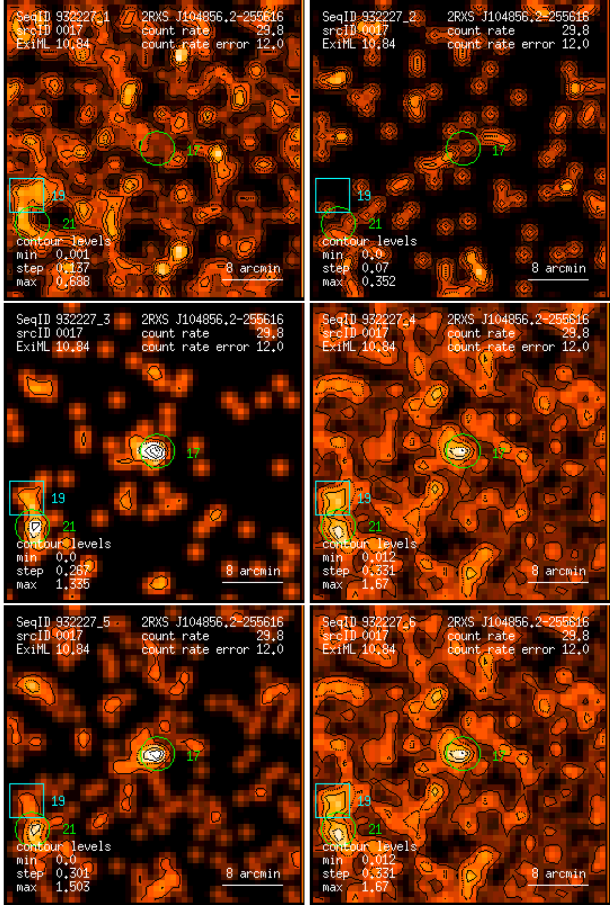
Figure 17: RASS 932227: detection 0017: band rate images, Gaussian filter: (1) PSPC channels 11 – 41, (2) 52 – 90, (3) 91 – 201, (4) 11 – 235, (5) 52 – 201, (6) 11 – 201. Broad band rates in counts/ks. Band rate contour levels in counts/ks/arcmin 2 .
