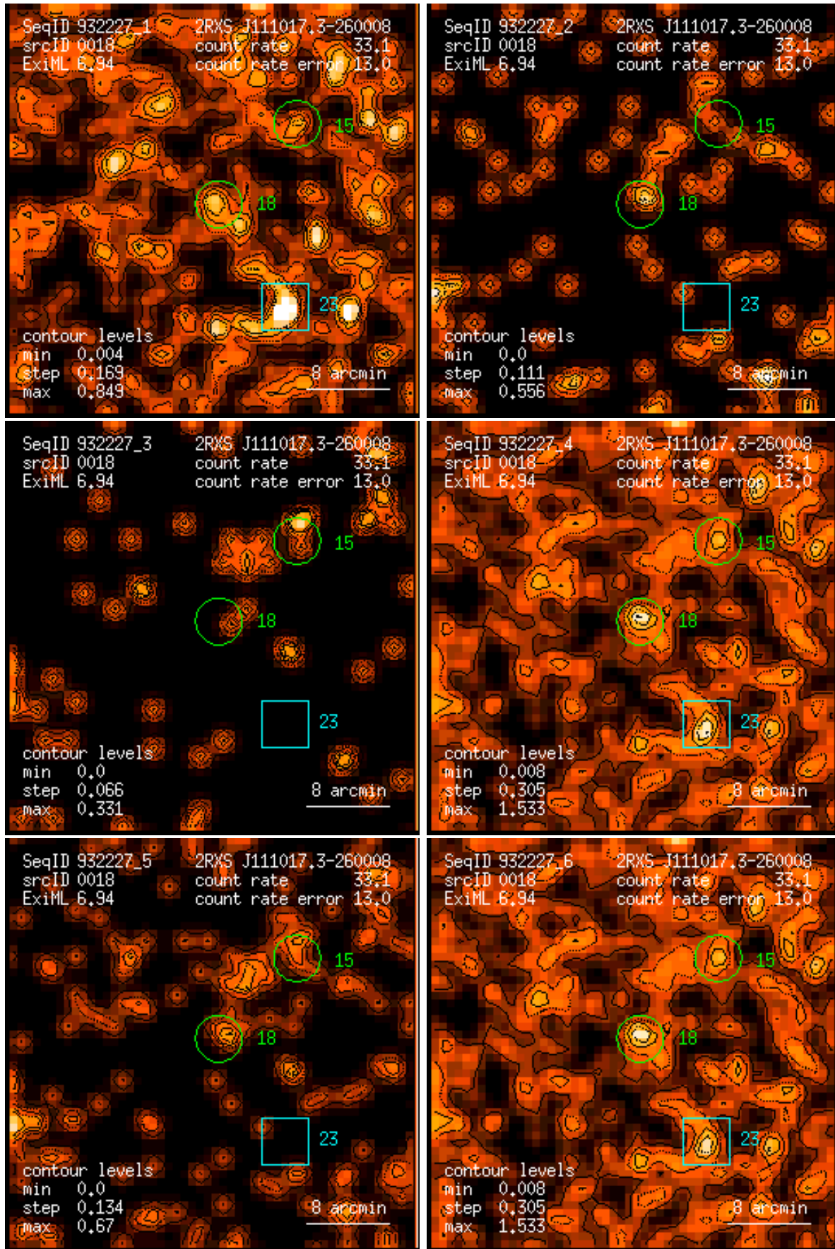
Figure 18: RASS 932227: detection 0018: band rate images, Gaussian filter: (1) PSPC channels 11 – 41, (2) 52 – 90, (3) 91 – 201, (4) 11 – 235, (5) 52 – 201, (6) 11 – 201. Broad band rates in counts/ks. Band rate contour levels in counts/ks/arcmin 2 .
