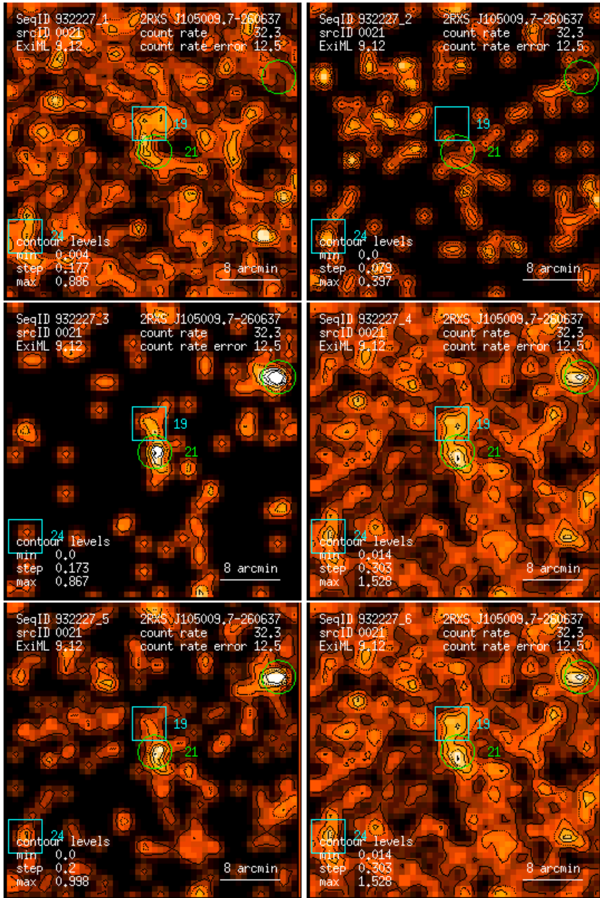
Figure 21: RASS 932227: detection 0021: band rate images, Gaussian filter: (1) PSPC channels 11 – 41, (2) 52 – 90, (3) 91 – 201, (4) 11 – 235, (5) 52 – 201, (6) 11 – 201. Broad band rates in counts/ks. Band rate contour levels in counts/ks/arcmin 2 .
