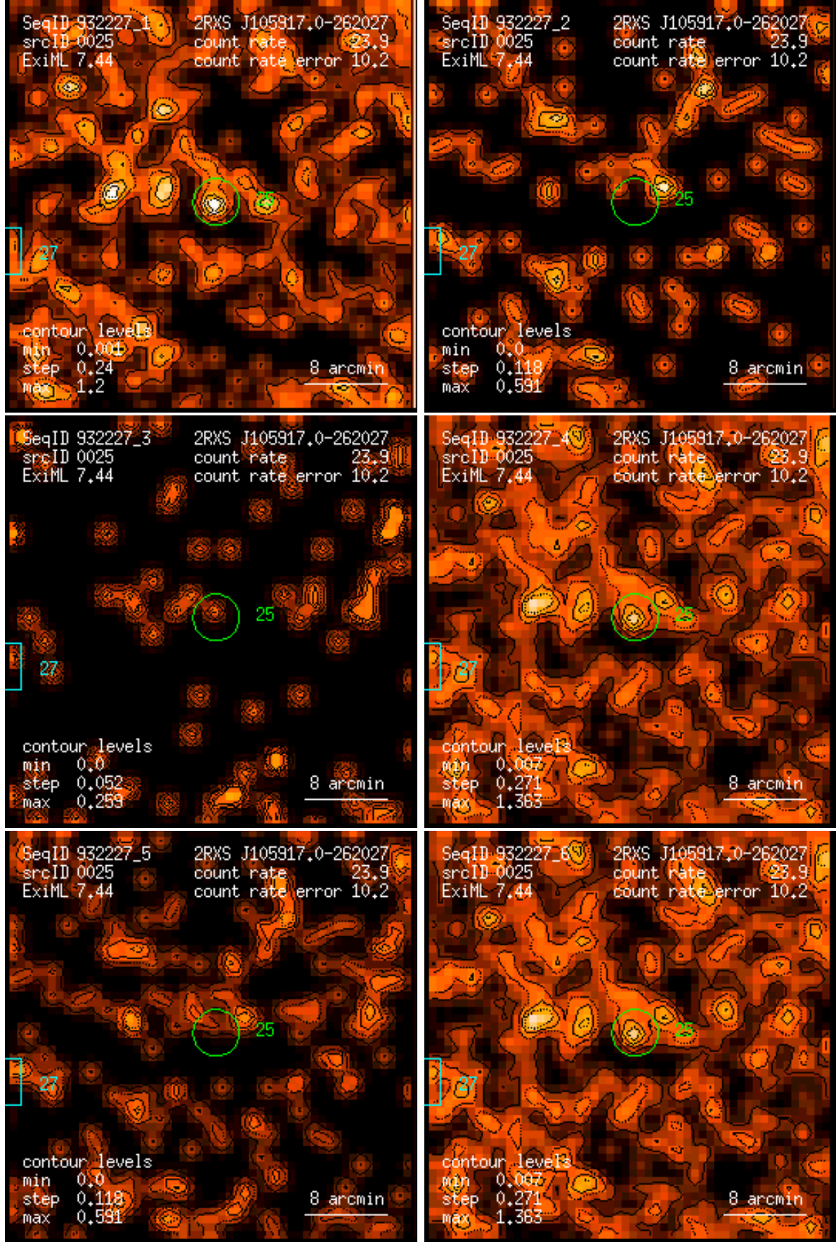
Figure 25: RASS 932227: detection 0025: band rate images, Gaussian filter: (1) PSPC channels 11 – 41, (2) 52 – 90, (3) 91 – 201, (4) 11 – 235, (5) 52 – 201, (6) 11 – 201. Broad band rates in counts/ks. Band rate contour levels in counts/ks/arcmin 2 .
