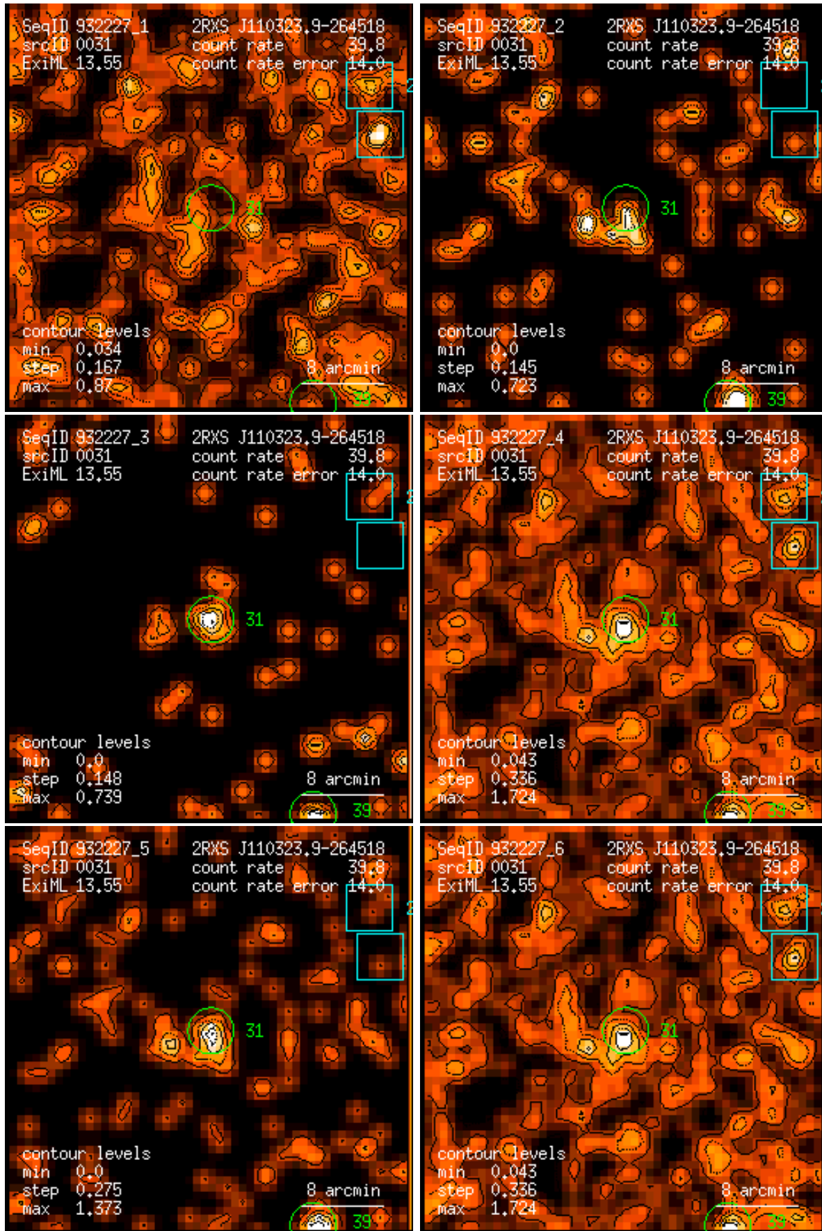
Figure 31: RASS 932227: detection 0031: band rate images, Gaussian filter: (1) PSPC channels 11 – 41, (2) 52 – 90, (3) 91 – 201, (4) 11 – 235, (5) 52 – 201, (6) 11 – 201. Broad band rates in counts/ks. Band rate contour levels in counts/ks/arcmin 2 .
