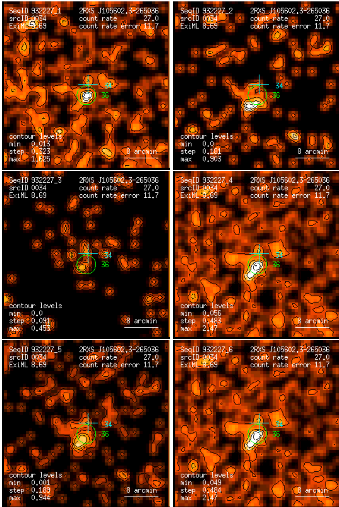
Figure 34: RASS 932227: detection 0034: band rate images, Gaussian filter: (1) PSPC channels 11 – 41, (2) 52 – 90, (3) 91 – 201, (4) 11 – 235, (5) 52 – 201, (6) 11 – 201. Broad band rates in counts/ks. Band rate contour levels in counts/ks/arcmin 2 .
