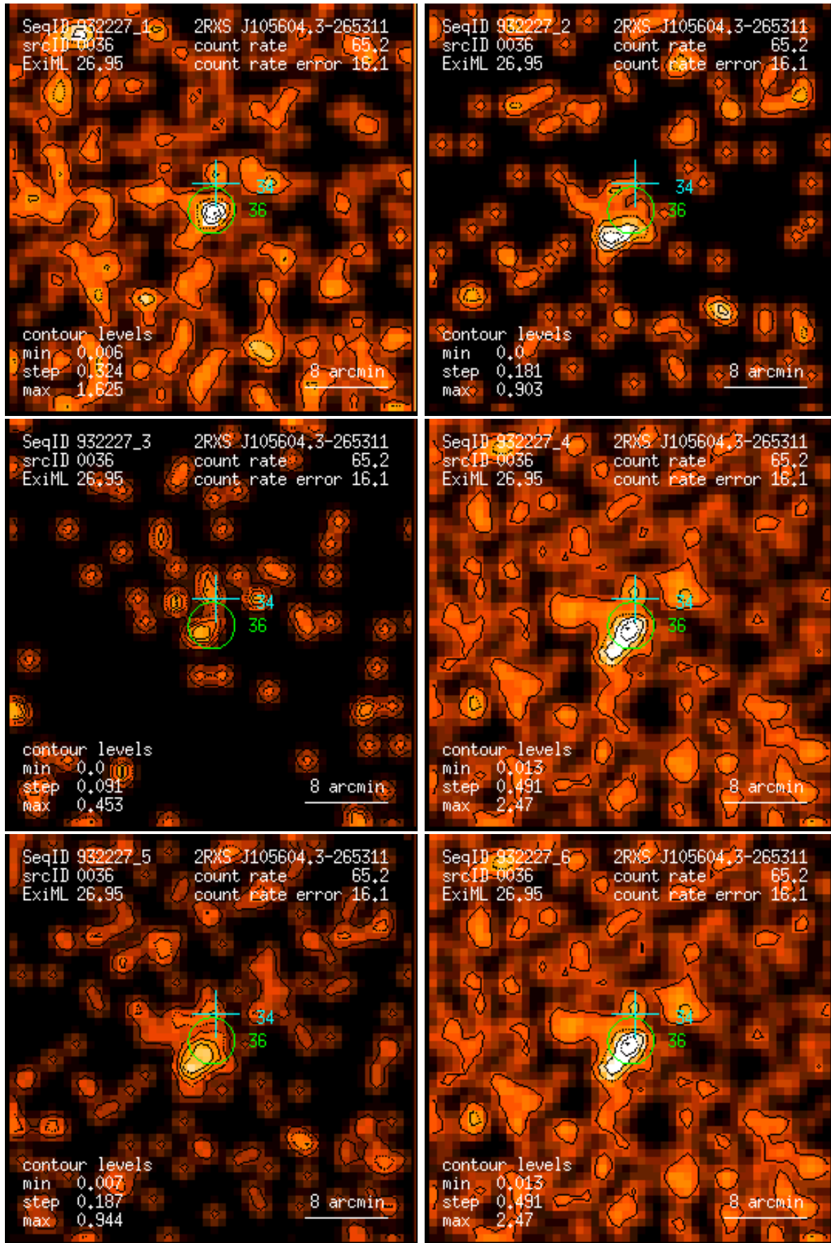
Figure 36: RASS 932227: detection 0036: band rate images, Gaussian filter: (1) PSPC channels 11 – 41, (2) 52 – 90, (3) 91 – 201, (4) 11 – 235, (5) 52 – 201, (6) 11 – 201. Broad band rates in counts/ks. Band rate contour levels in counts/ks/arcmin 2 .
