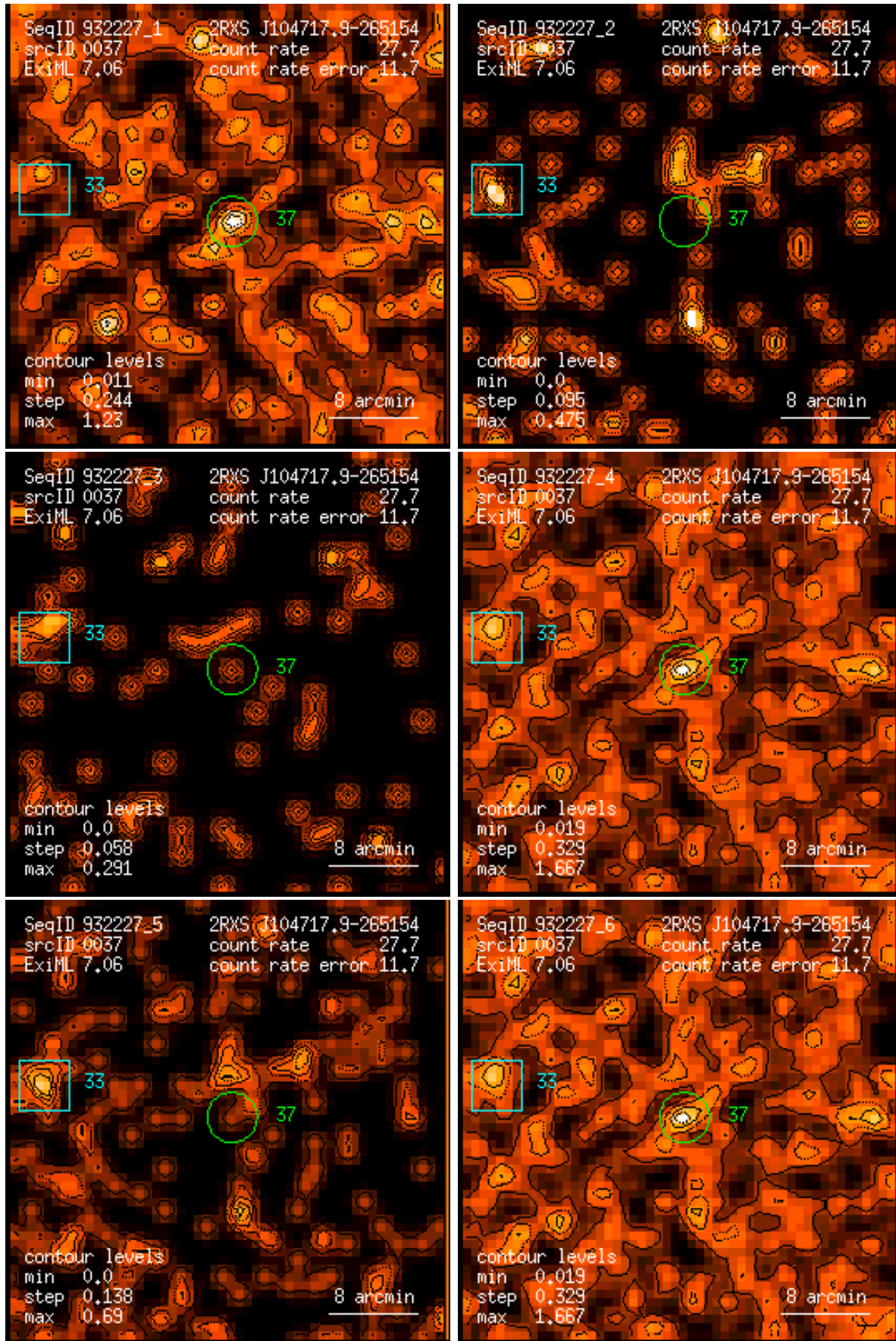
Figure 37: RASS 932227: detection 0037: band rate images, Gaussian filter: (1) PSPC channels 11 – 41, (2) 52 – 90, (3) 91 – 201, (4) 11 – 235, (5) 52 – 201, (6) 11 – 201. Broad band rates in counts/ks. Band rate contour levels in counts/ks/arcmin 2 .
