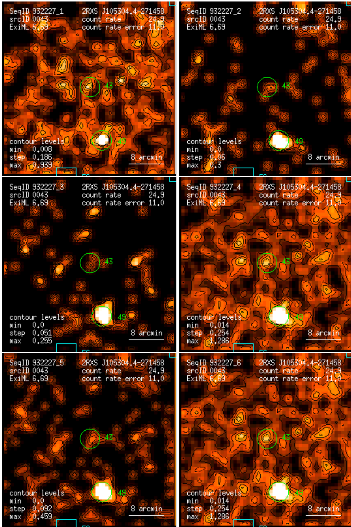
Figure 43: RASS 932227: detection 0043: band rate images, Gaussian filter: (1) PSPC channels 11 – 41, (2) 52 – 90, (3) 91 – 201, (4) 11 – 235, (5) 52 – 201, (6) 11 – 201. Broad band rates in counts/ks. Band rate contour levels in counts/ks/arcmin 2 .
