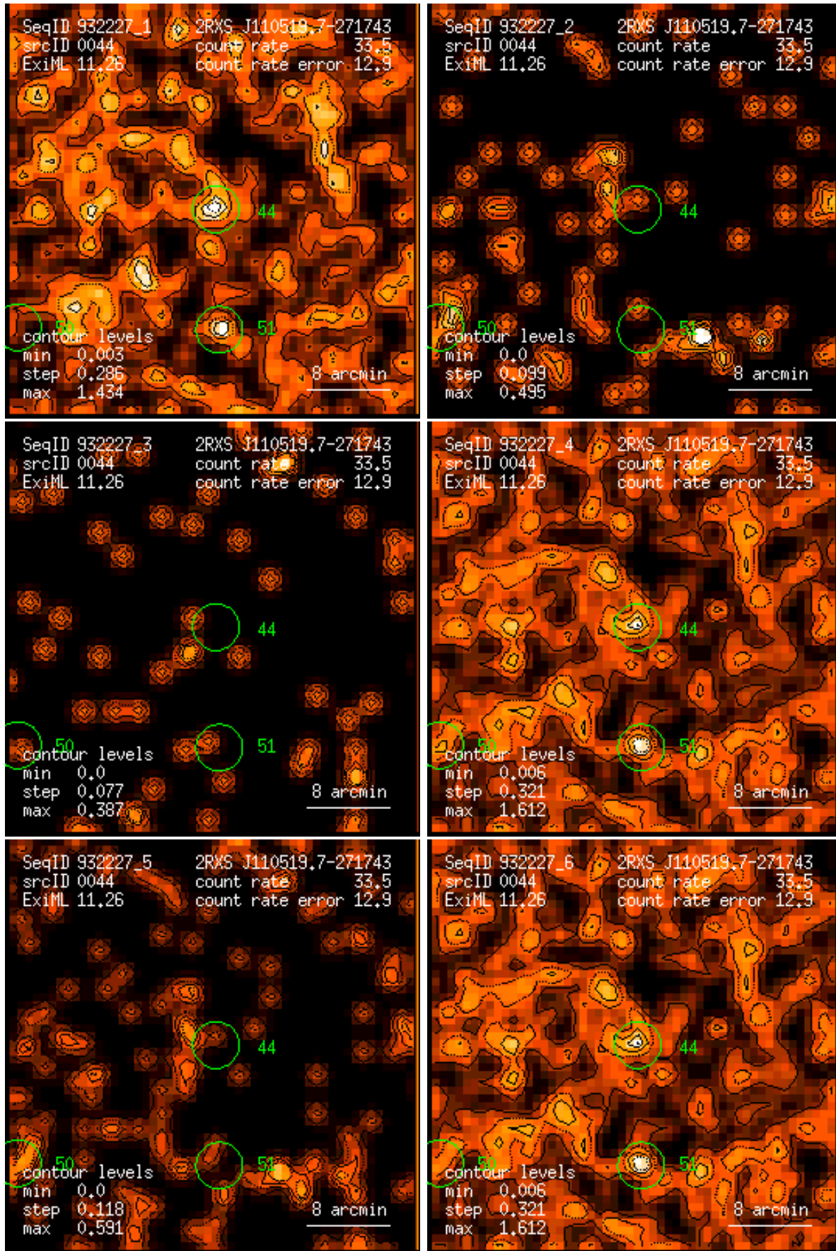
Figure 44: RASS 932227: detection 0044: band rate images, Gaussian filter: (1) PSPC channels 11 – 41, (2) 52 – 90, (3) 91 – 201, (4) 11 – 235, (5) 52 – 201, (6) 11 – 201. Broad band rates in counts/ks. Band rate contour levels in counts/ks/arcmin 2 .
