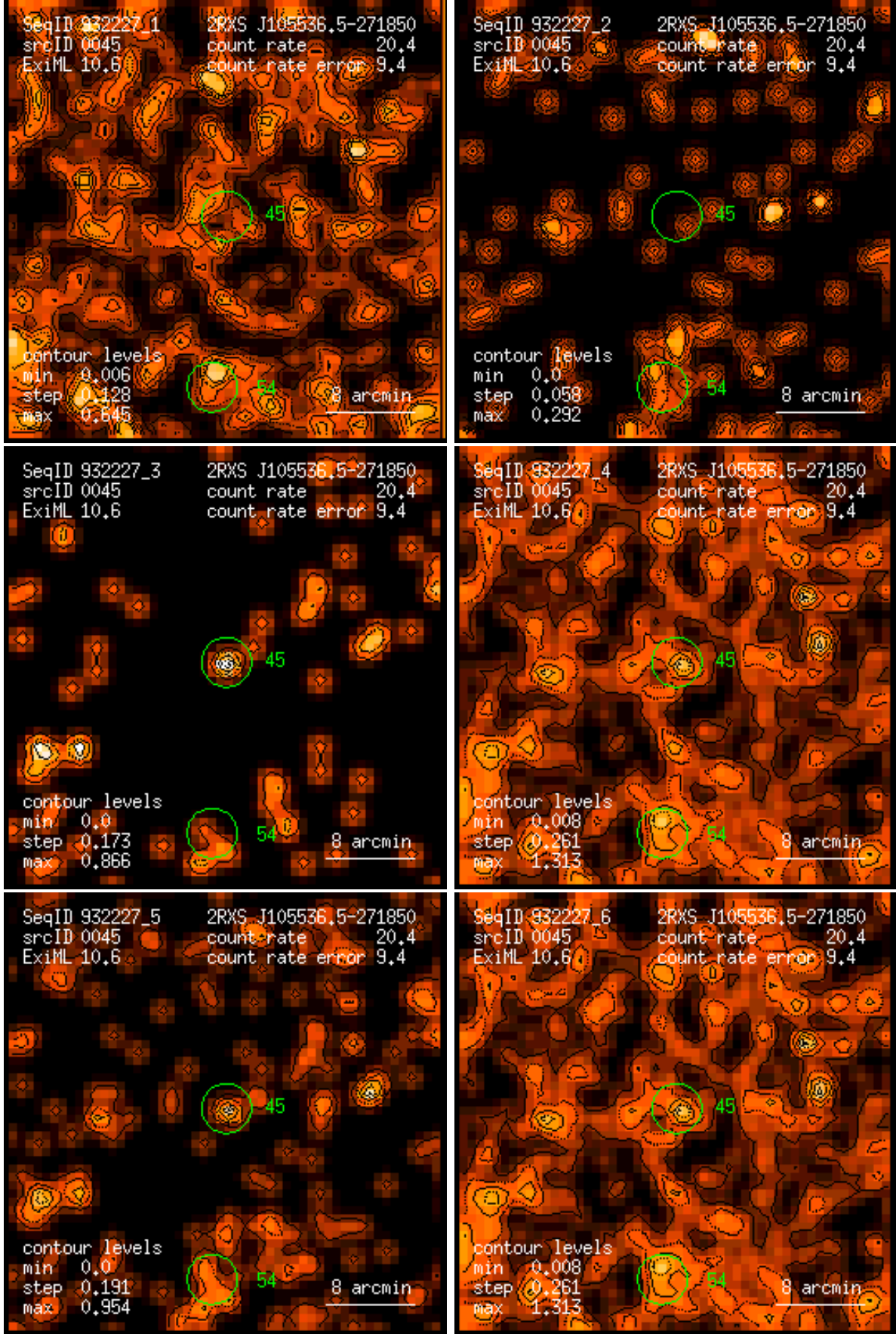
Figure 45: RASS 932227: detection 0045: band rate images, Gaussian filter: (1) PSPC channels 11 – 41, (2) 52 – 90, (3) 91 – 201, (4) 11 – 235, (5) 52 – 201, (6) 11 – 201. Broad band rates in counts/ks. Band rate contour levels in counts/ks/arcmin 2 .
