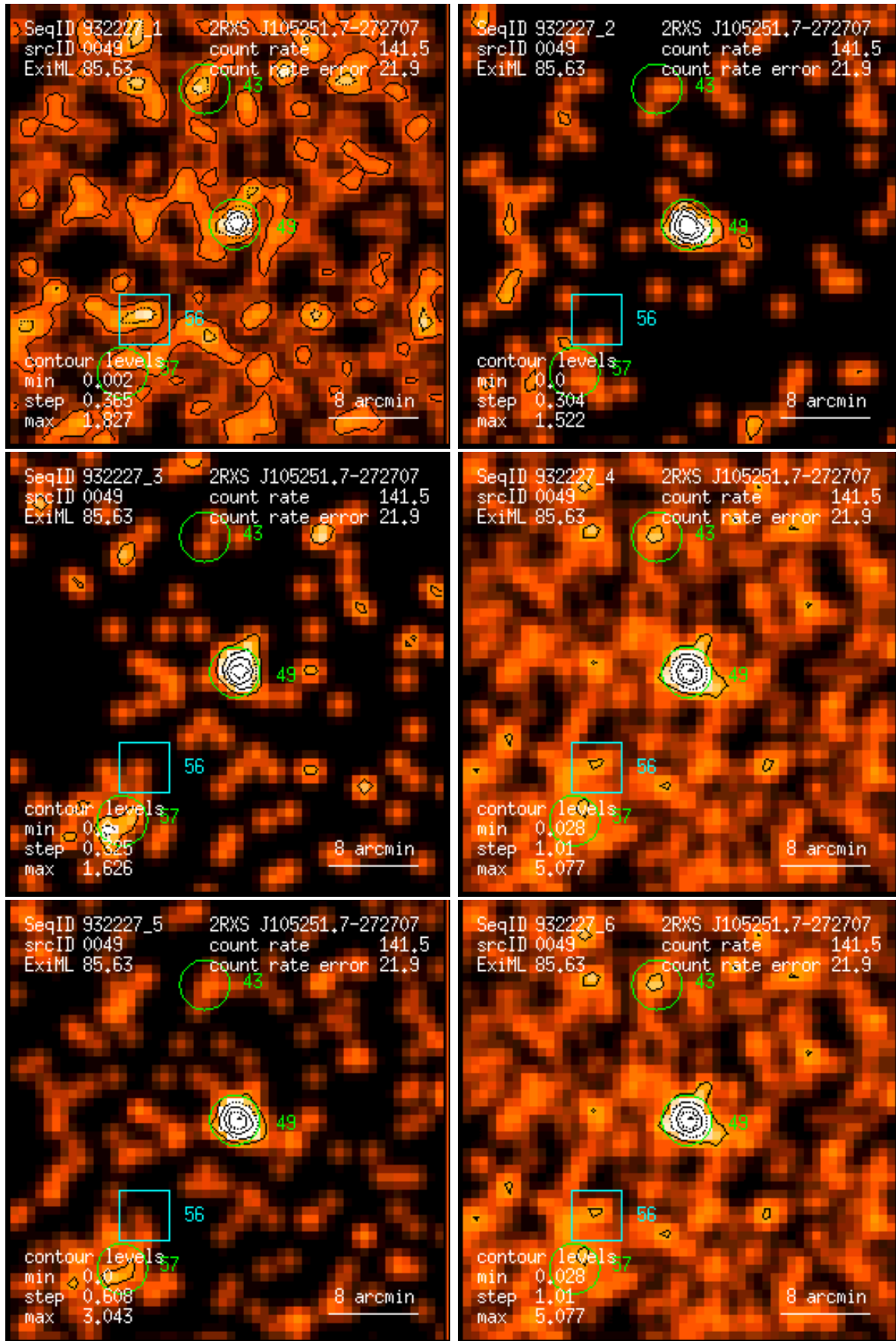
Figure 49: RASS 932227: detection 0049: band rate images, Gaussian filter: (1) PSPC channels 11 – 41, (2) 52 – 90, (3) 91 – 201, (4) 11 – 235, (5) 52 – 201, (6) 11 – 201. Broad band rates in counts/ks. Band rate contour levels in counts/ks/arcmin 2 .
