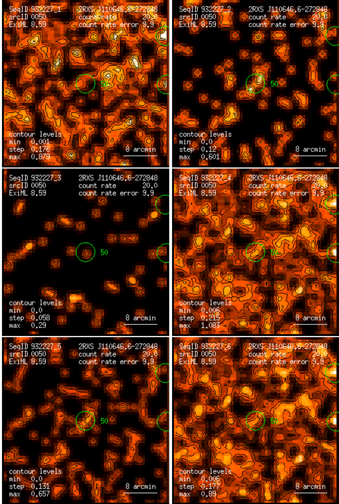
Figure 50: RASS 932227: detection 0050: band rate images, Gaussian filter: (1) PSPC channels 11 – 41, (2) 52 – 90, (3) 91 – 201, (4) 11 – 235, (5) 52 – 201, (6) 11 – 201. Broad band rates in counts/ks. Band rate contour levels in counts/ks/arcmin 2 .
