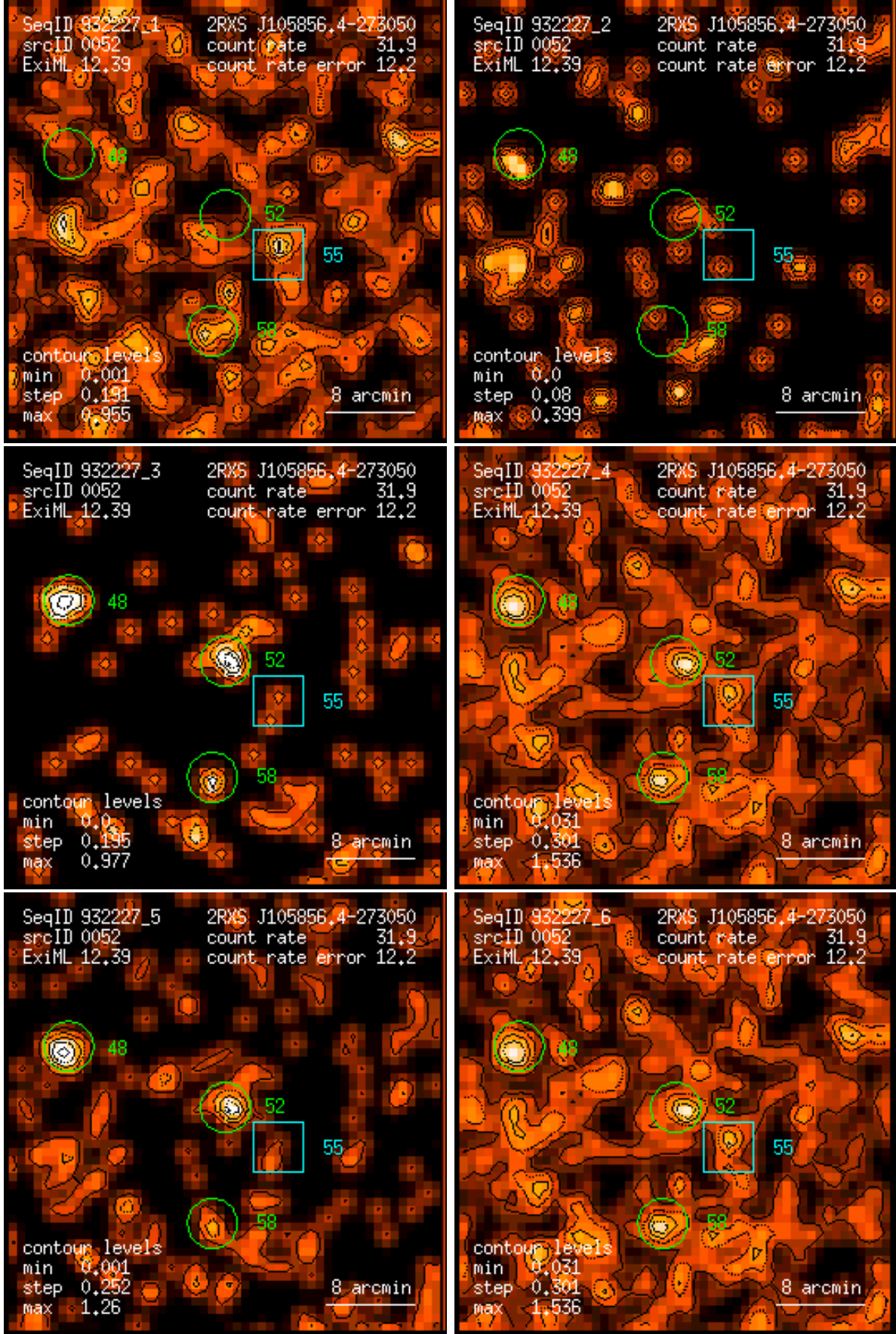
Figure 52: RASS 932227: detection 0052: band rate images, Gaussian filter: (1) PSPC channels 11 – 41, (2) 52 – 90, (3) 91 – 201, (4) 11 – 235, (5) 52 – 201, (6) 11 – 201. Broad band rates in counts/ks. Band rate contour levels in counts/ks/arcmin 2 .
