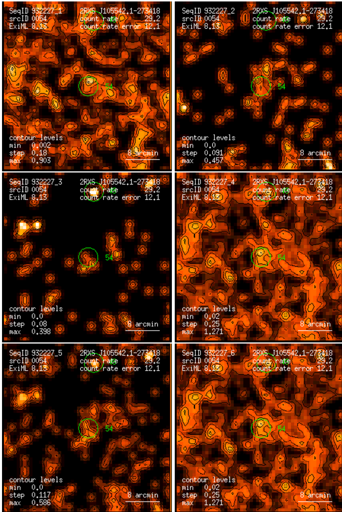
Figure 54: RASS 932227: detection 0054: band rate images, Gaussian filter: (1) PSPC channels 11 – 41, (2) 52 – 90, (3) 91 – 201, (4) 11 – 235, (5) 52 – 201, (6) 11 – 201. Broad band rates in counts/ks. Band rate contour levels in counts/ks/arcmin 2 .
