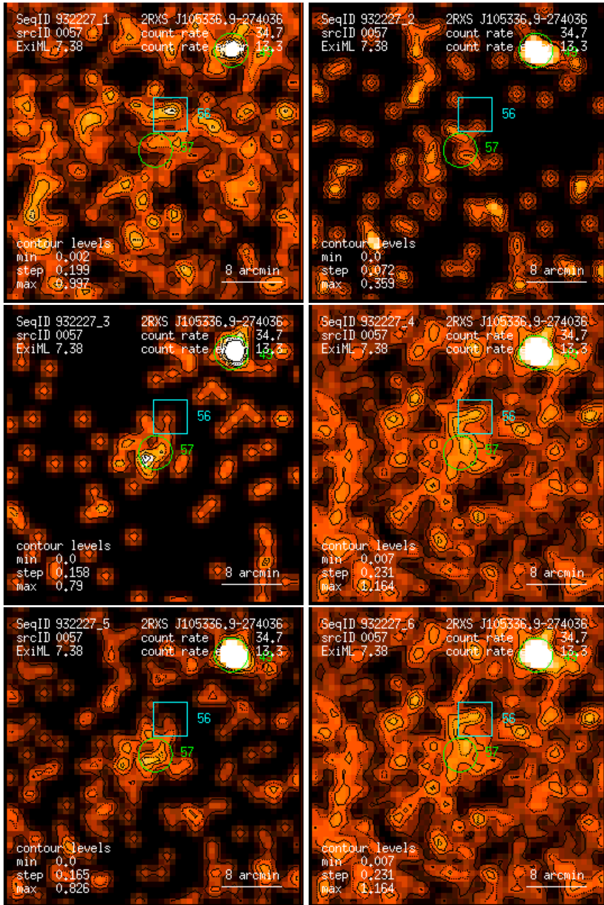
Figure 57: RASS 932227: detection 0057: band rate images, Gaussian filter: (1) PSPC channels 11 – 41, (2) 52 – 90, (3) 91 – 201, (4) 11 – 235, (5) 52 – 201, (6) 11 – 201. Broad band rates in counts/ks. Band rate contour levels in counts/ks/arcmin 2 .
