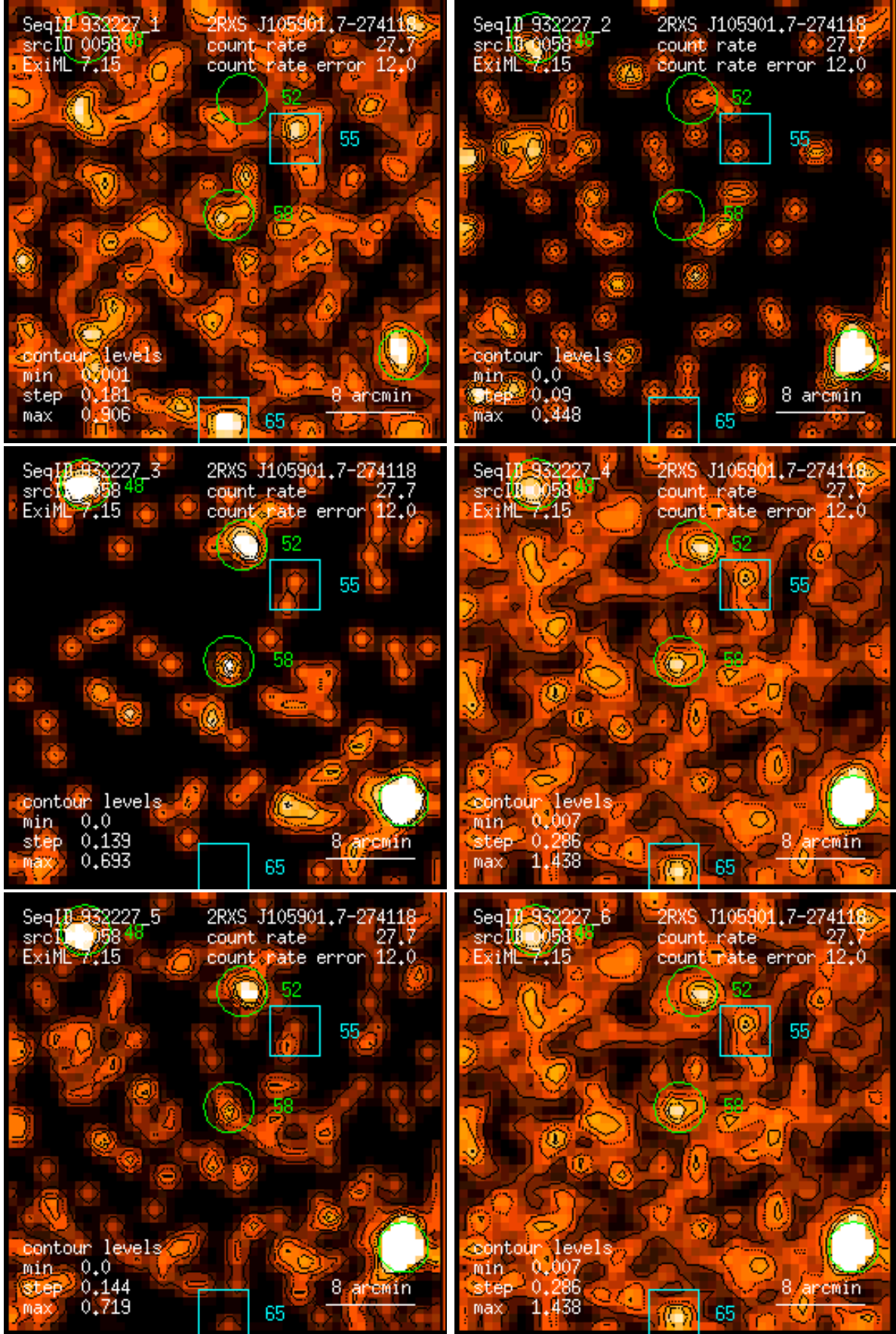
Figure 58: RASS 932227: detection 0058: band rate images, Gaussian filter: (1) PSPC channels 11 – 41, (2) 52 – 90, (3) 91 – 201, (4) 11 – 235, (5) 52 – 201, (6) 11 – 201. Broad band rates in counts/ks. Band rate contour levels in counts/ks/arcmin 2 .
