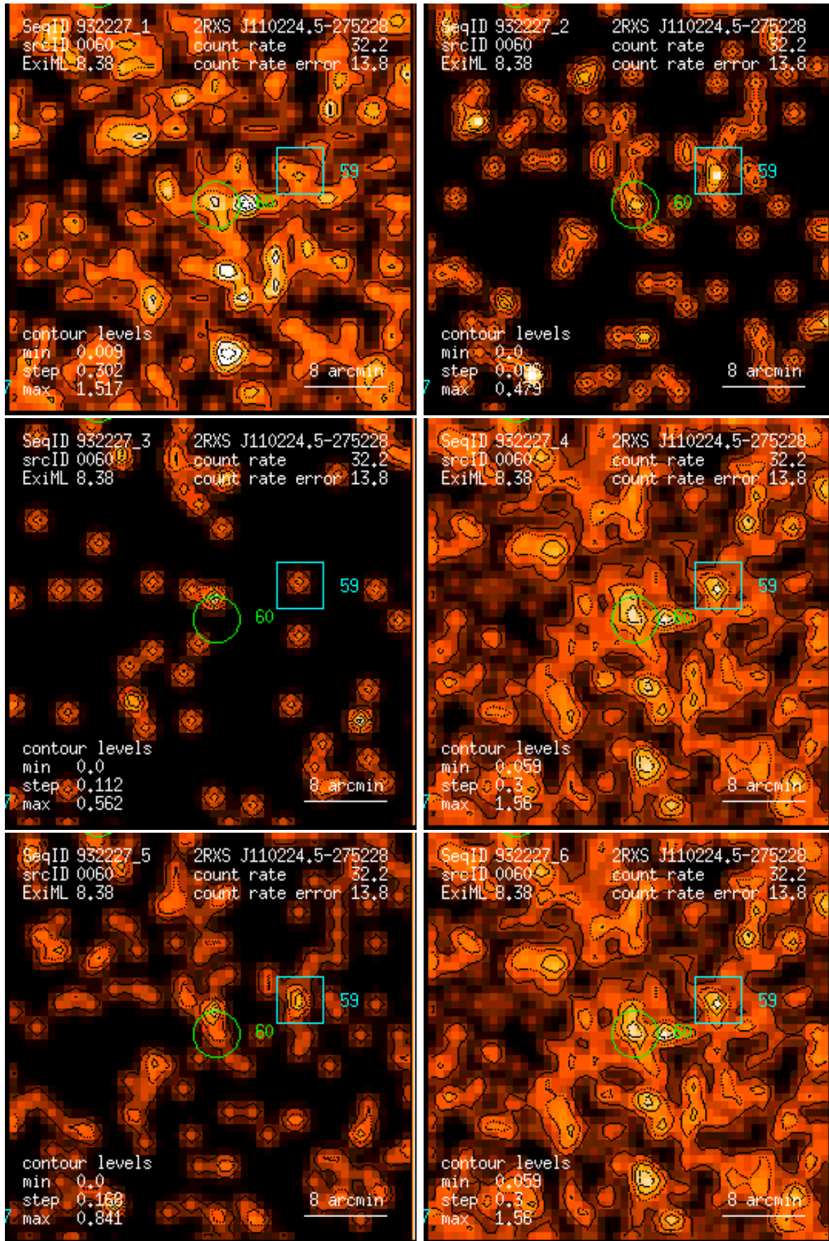
Figure 60: RASS 932227: detection 0060: band rate images, Gaussian filter: (1) PSPC channels 11 – 41, (2) 52 – 90, (3) 91 – 201, (4) 11 – 235, (5) 52 – 201, (6) 11 – 201. Broad band rates in counts/ks. Band rate contour levels in counts/ks/arcmin 2 .
