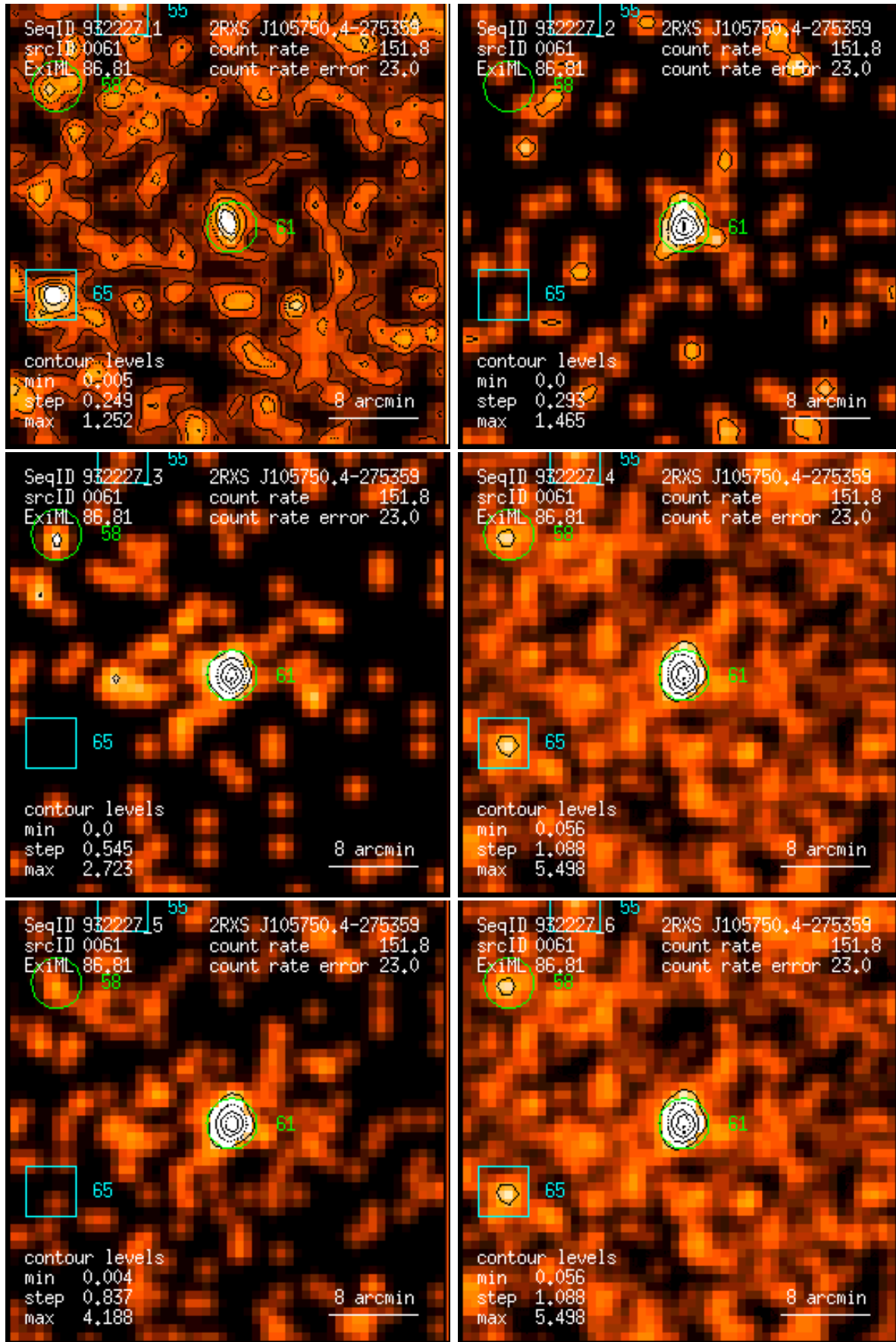
Figure 61: RASS 932227: detection 0061: band rate images, Gaussian filter: (1) PSPC channels 11 – 41, (2) 52 – 90, (3) 91 – 201, (4) 11 – 235, (5) 52 – 201, (6) 11 – 201. Broad band rates in counts/ks. Band rate contour levels in counts/ks/arcmin 2 .
