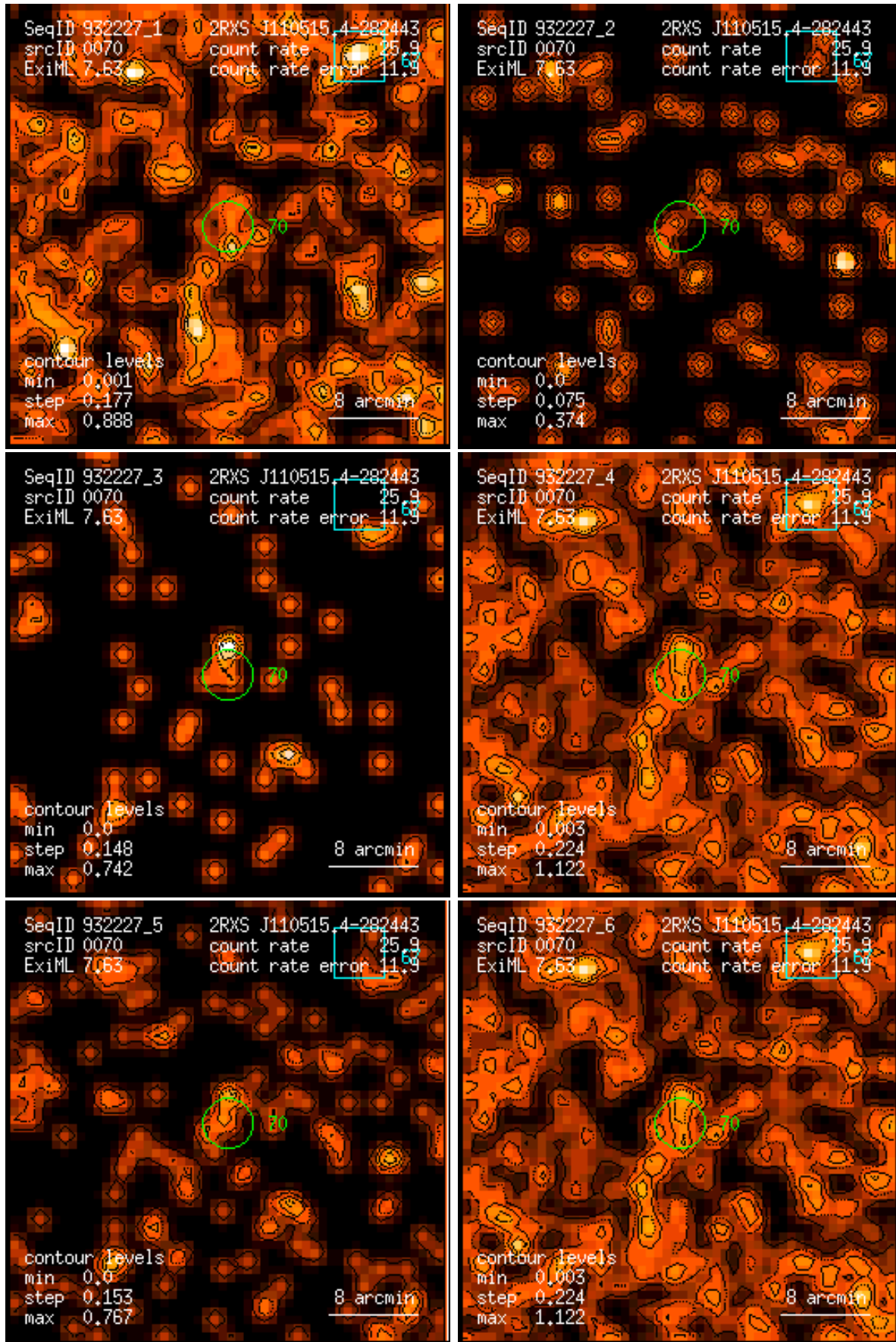
Figure 70: RASS 932227: detection 0070: band rate images, Gaussian filter: (1) PSPC channels 11 – 41, (2) 52 – 90, (3) 91 – 201, (4) 11 – 235, (5) 52 – 201, (6) 11 – 201. Broad band rates in counts/ks. Band rate contour levels in counts/ks/arcmin 2 .
