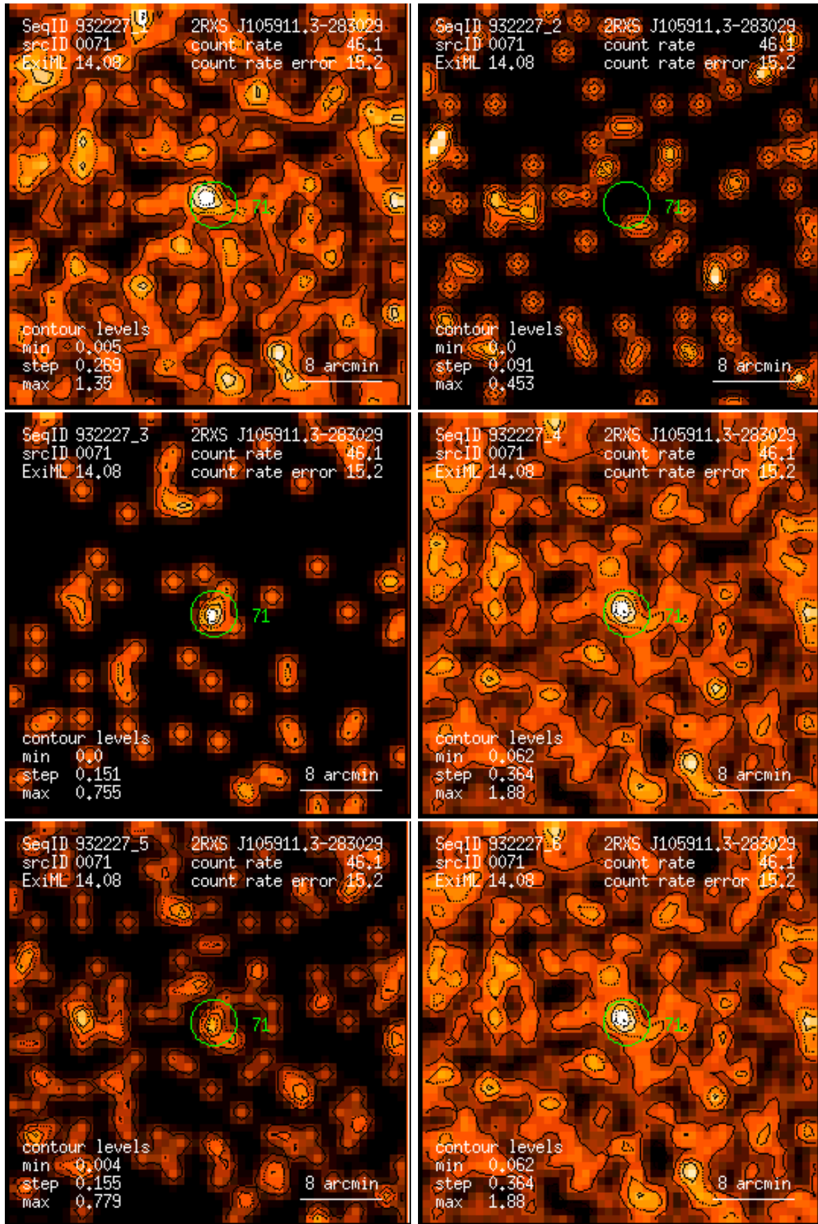
Figure 71: RASS 932227: detection 0071: band rate images, Gaussian filter: (1) PSPC channels 11 – 41, (2) 52 – 90, (3) 91 – 201, (4) 11 – 235, (5) 52 – 201, (6) 11 – 201. Broad band rates in counts/ks. Band rate contour levels in counts/ks/arcmin 2 .
