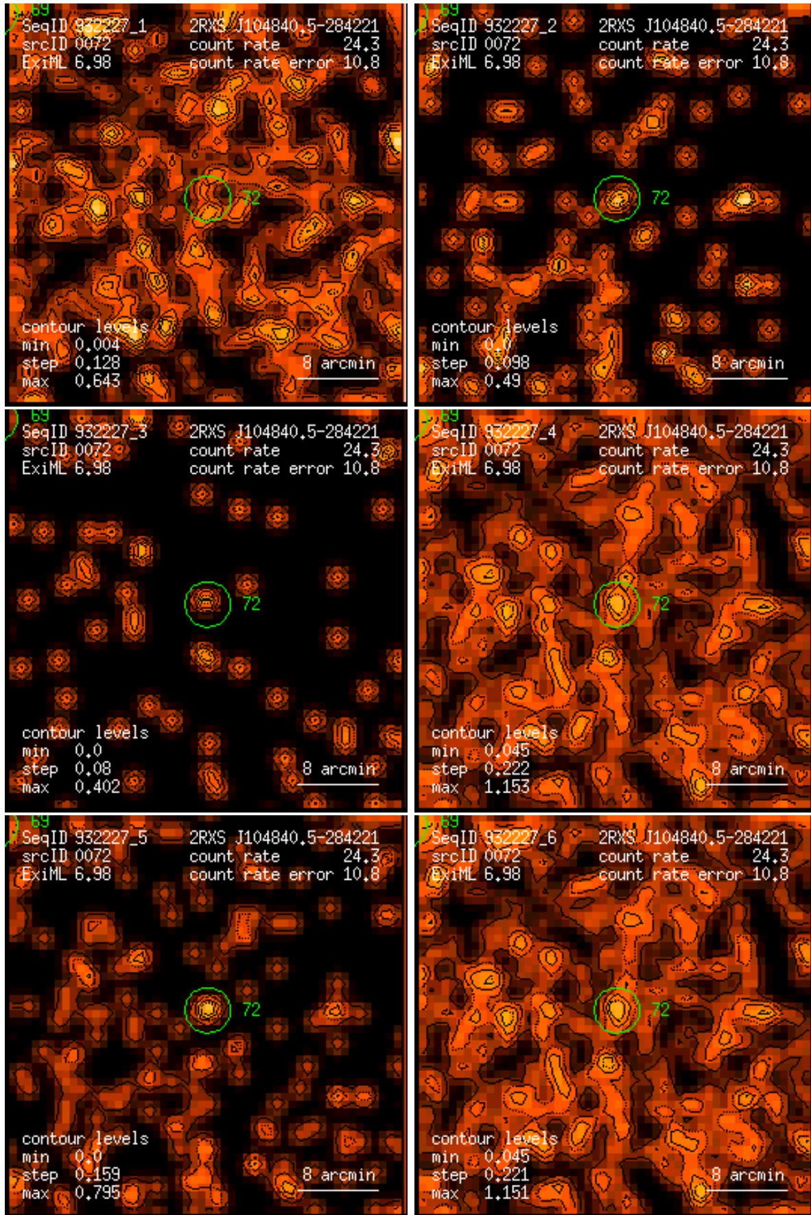
Figure 72: RASS 932227: detection 0072: band rate images, Gaussian filter: (1) PSPC channels 11 – 41, (2) 52 – 90, (3) 91 – 201, (4) 11 – 235, (5) 52 – 201, (6) 11 – 201. Broad band rates in counts/ks. Band rate contour levels in counts/ks/arcmin 2 .
