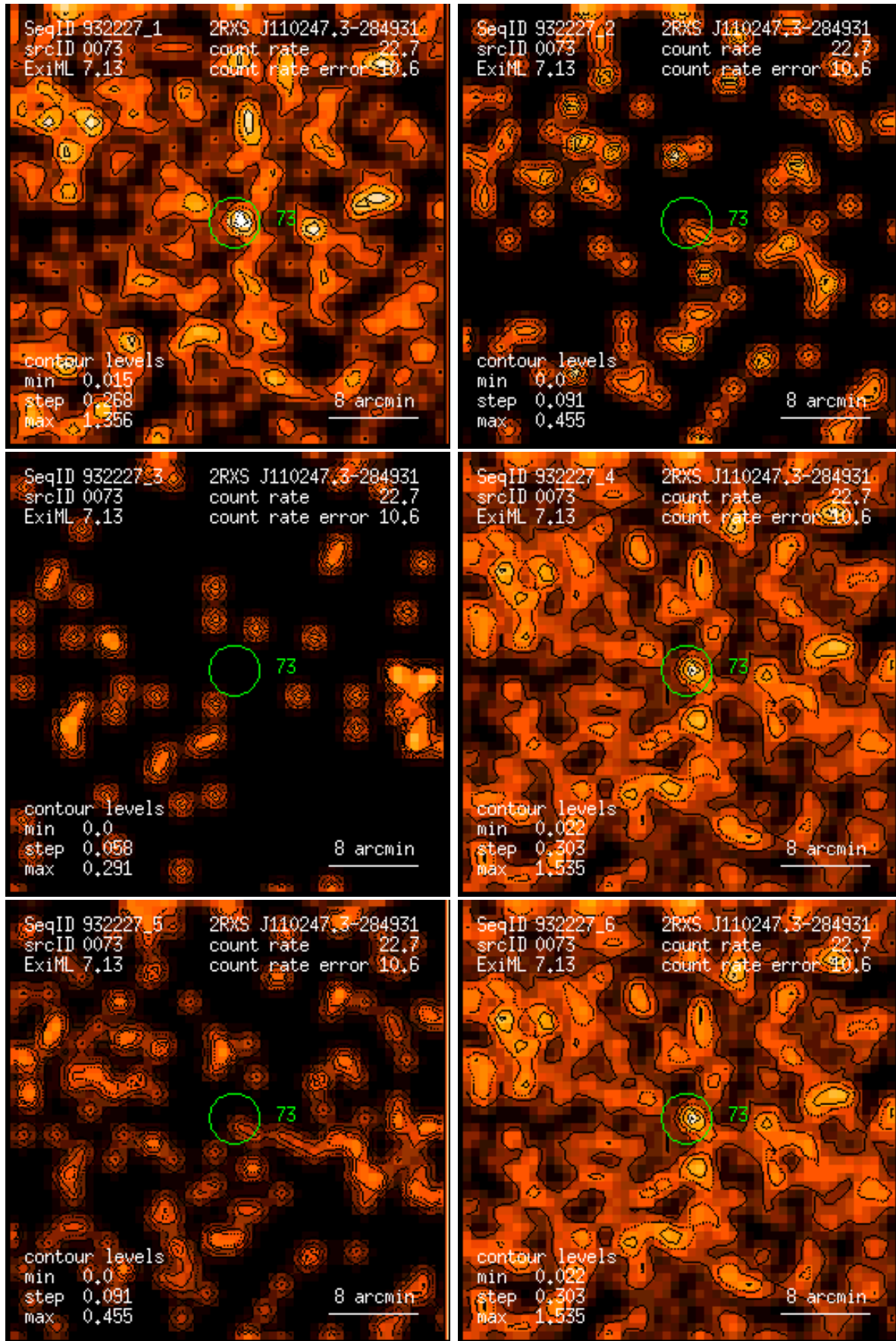
Figure 73: RASS 932227: detection 0073: band rate images, Gaussian filter: (1) PSPC channels 11 – 41, (2) 52 – 90, (3) 91 – 201, (4) 11 – 235, (5) 52 – 201, (6) 11 – 201. Broad band rates in counts/ks. Band rate contour levels in counts/ks/arcmin 2 .
