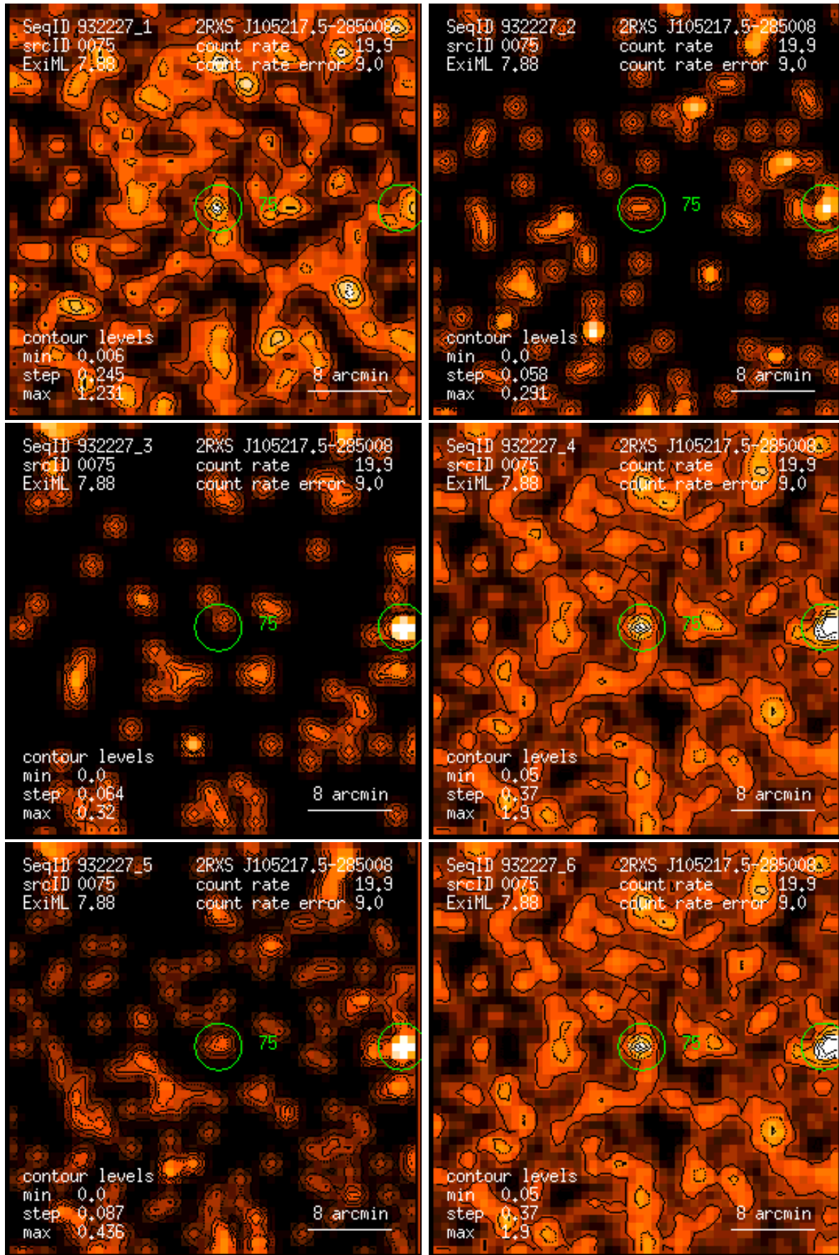
Figure 75: RASS 932227: detection 0075: band rate images, Gaussian filter: (1) PSPC channels 11 – 41, (2) 52 – 90, (3) 91 – 201, (4) 11 – 235, (5) 52 – 201, (6) 11 – 201. Broad band rates in counts/ks. Band rate contour levels in counts/ks/arcmin 2 .
