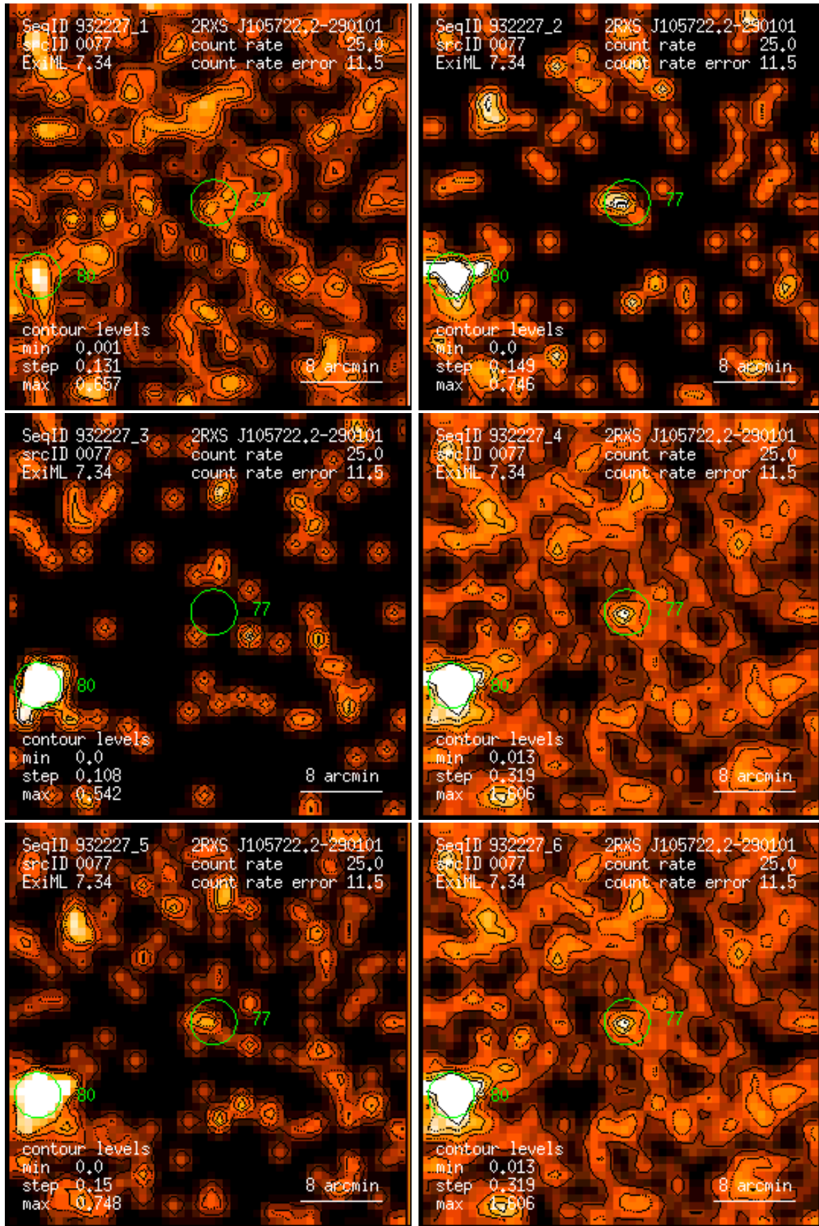
Figure 77: RASS 932227: detection 0077: band rate images, Gaussian filter: (1) PSPC channels 11 – 41, (2) 52 – 90, (3) 91 – 201, (4) 11 – 235, (5) 52 – 201, (6) 11 – 201. Broad band rates in counts/ks. Band rate contour levels in counts/ks/arcmin 2 .
