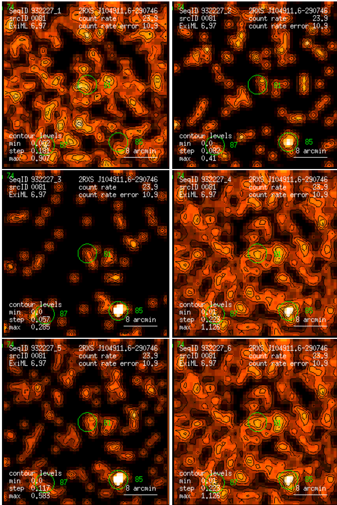
Figure 81: RASS 932227: detection 0081: band rate images, Gaussian filter: (1) PSPC channels 11 – 41, (2) 52 – 90, (3) 91 – 201, (4) 11 – 235, (5) 52 – 201, (6) 11 – 201. Broad band rates in counts/ks. Band rate contour levels in counts/ks/arcmin 2 .
