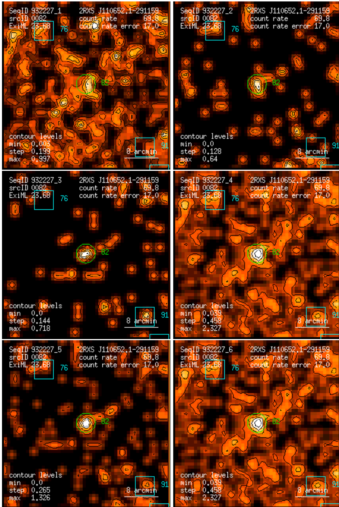
Figure 82: RASS 932227: detection 0082: band rate images, Gaussian filter: (1) PSPC channels 11 – 41, (2) 52 – 90, (3) 91 – 201, (4) 11 – 235, (5) 52 – 201, (6) 11 – 201. Broad band rates in counts/ks. Band rate contour levels in counts/ks/arcmin 2 .
