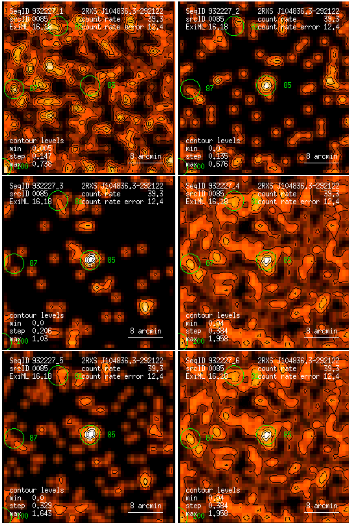
Figure 85: RASS 932227: detection 0085: band rate images, Gaussian filter: (1) PSPC channels 11 – 41, (2) 52 – 90, (3) 91 – 201, (4) 11 – 235, (5) 52 – 201, (6) 11 – 201. Broad band rates in counts/ks. Band rate contour levels in counts/ks/arcmin 2 .
