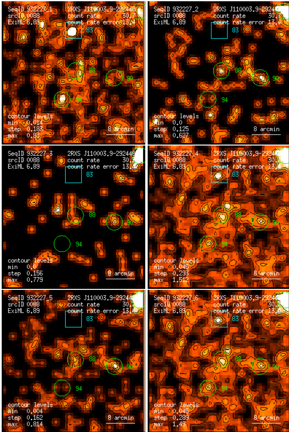
Figure 88: RASS 932227: detection 0088: band rate images, Gaussian filter: (1) PSPC channels 11 – 41, (2) 52 – 90, (3) 91 – 201, (4) 11 – 235, (5) 52 – 201, (6) 11 – 201. Broad band rates in counts/ks. Band rate contour levels in counts/ks/arcmin 2 .
