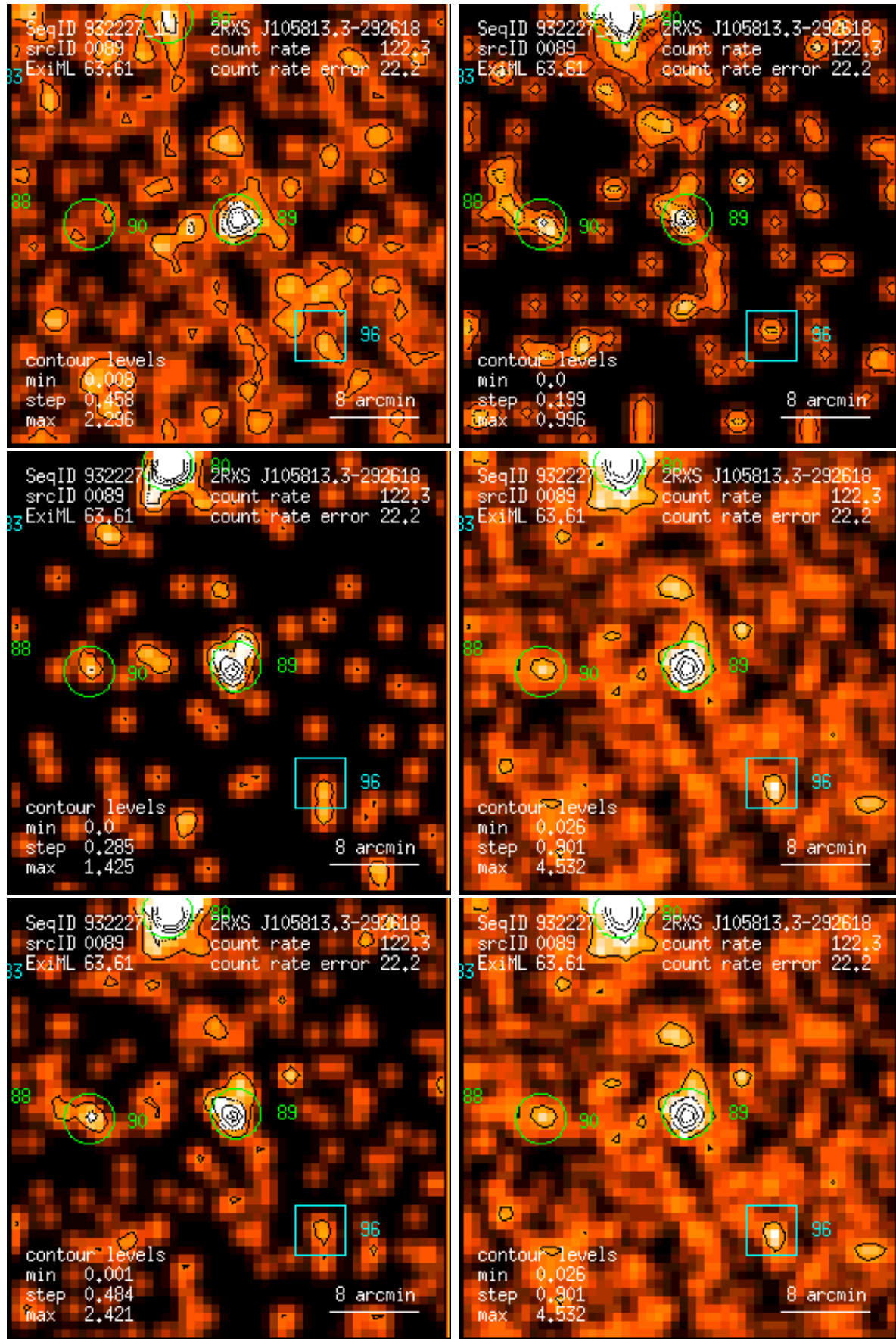
Figure 89: RASS 932227: detection 0089: band rate images, Gaussian filter: (1) PSPC channels 11 – 41, (2) 52 – 90, (3) 91 – 201, (4) 11 – 235, (5) 52 – 201, (6) 11 – 201. Broad band rates in counts/ks. Band rate contour levels in counts/ks/arcmin 2 .
