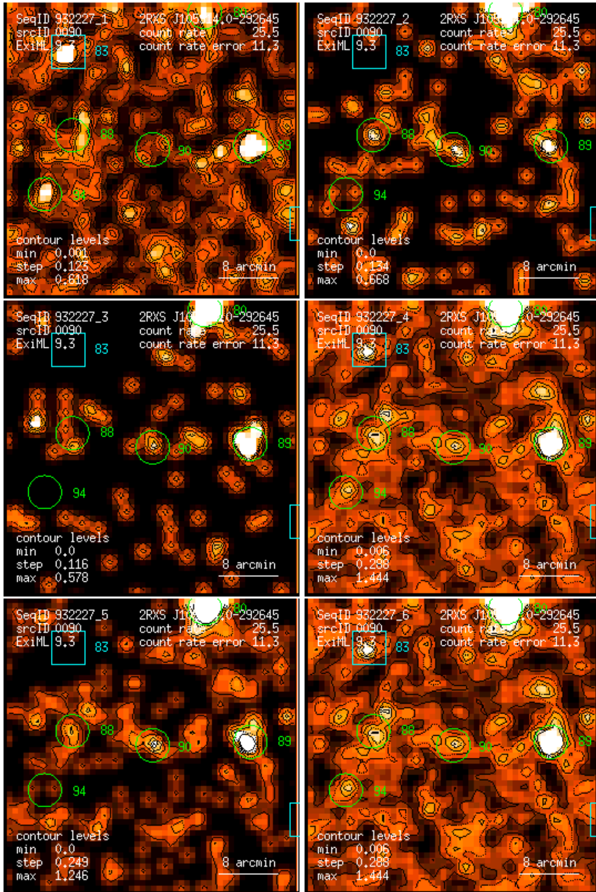
Figure 90: RASS 932227: detection 0090: band rate images, Gaussian filter: (1) PSPC channels 11 – 41, (2) 52 – 90, (3) 91 – 201, (4) 11 – 235, (5) 52 – 201, (6) 11 – 201. Broad band rates in counts/ks. Band rate contour levels in counts/ks/arcmin 2 .
