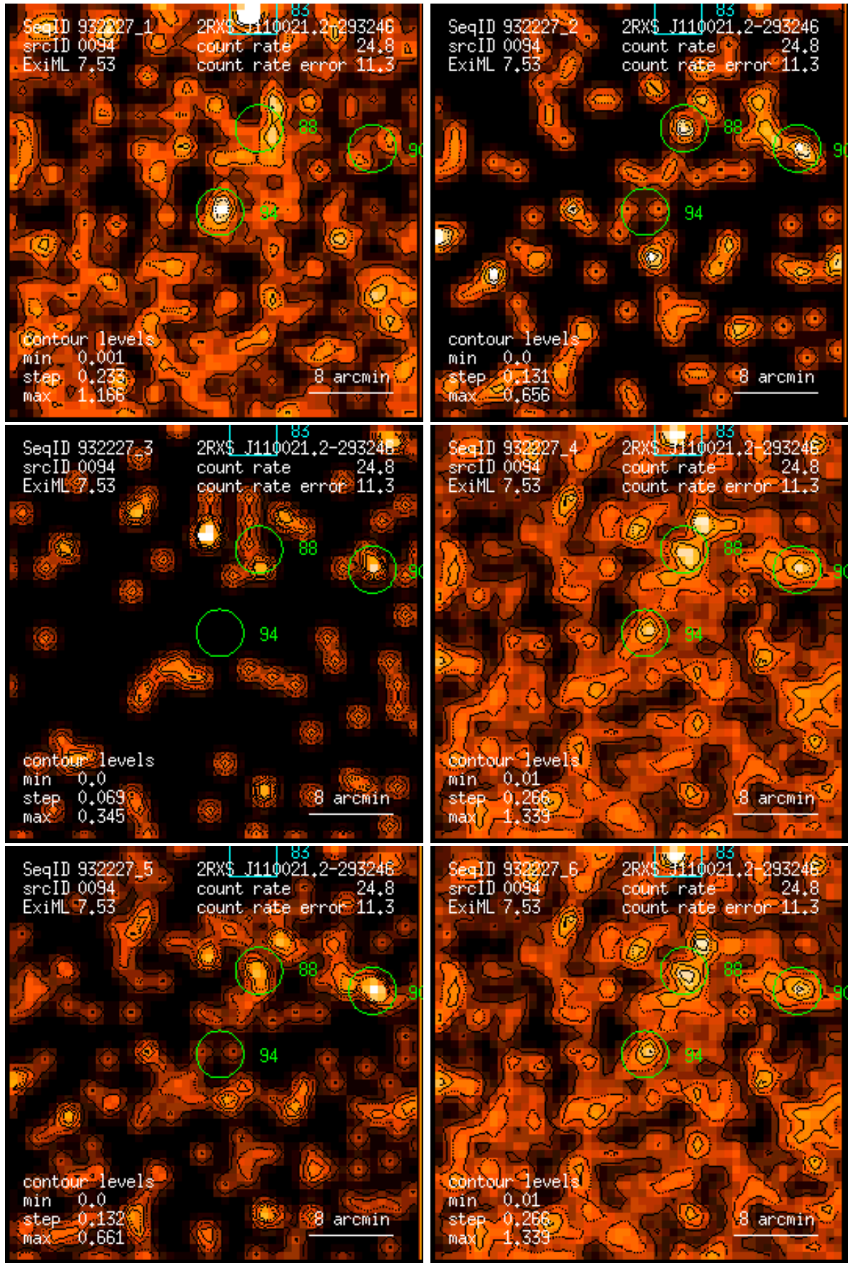
Figure 94: RASS 932227: detection 0094: band rate images, Gaussian filter: (1) PSPC channels 11 – 41, (2) 52 – 90, (3) 91 – 201, (4) 11 – 235, (5) 52 – 201, (6) 11 – 201. Broad band rates in counts/ks. Band rate contour levels in counts/ks/arcmin 2 .
