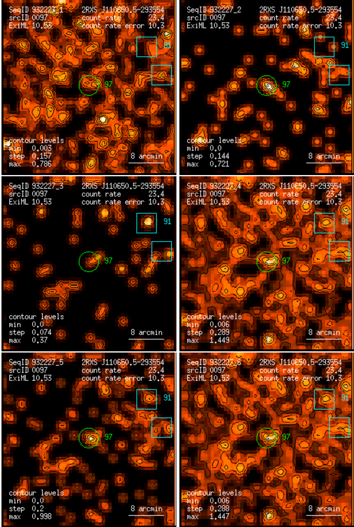
Figure 97: RASS 932227: detection 0097: band rate images, Gaussian filter: (1) PSPC channels 11 – 41, (2) 52 – 90, (3) 91 – 201, (4) 11 – 235, (5) 52 – 201, (6) 11 – 201. Broad band rates in counts/ks. Band rate contour levels in counts/ks/arcmin 2 .
