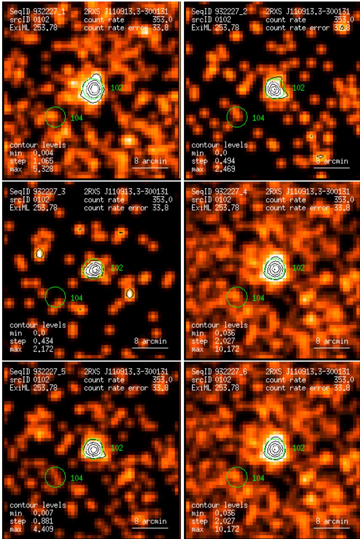
Figure 102: RASS 932227: detection 0102: band rate images, Gaussian filter: (1) PSPC channels 11 – 41, (2) 52 – 90, (3) 91 – 201, (4) 11 – 235, (5) 52 – 201, (6) 11 – 201. Broad band rates in counts/ks. Band rate contour levels in counts/ks/arcmin 2 .
