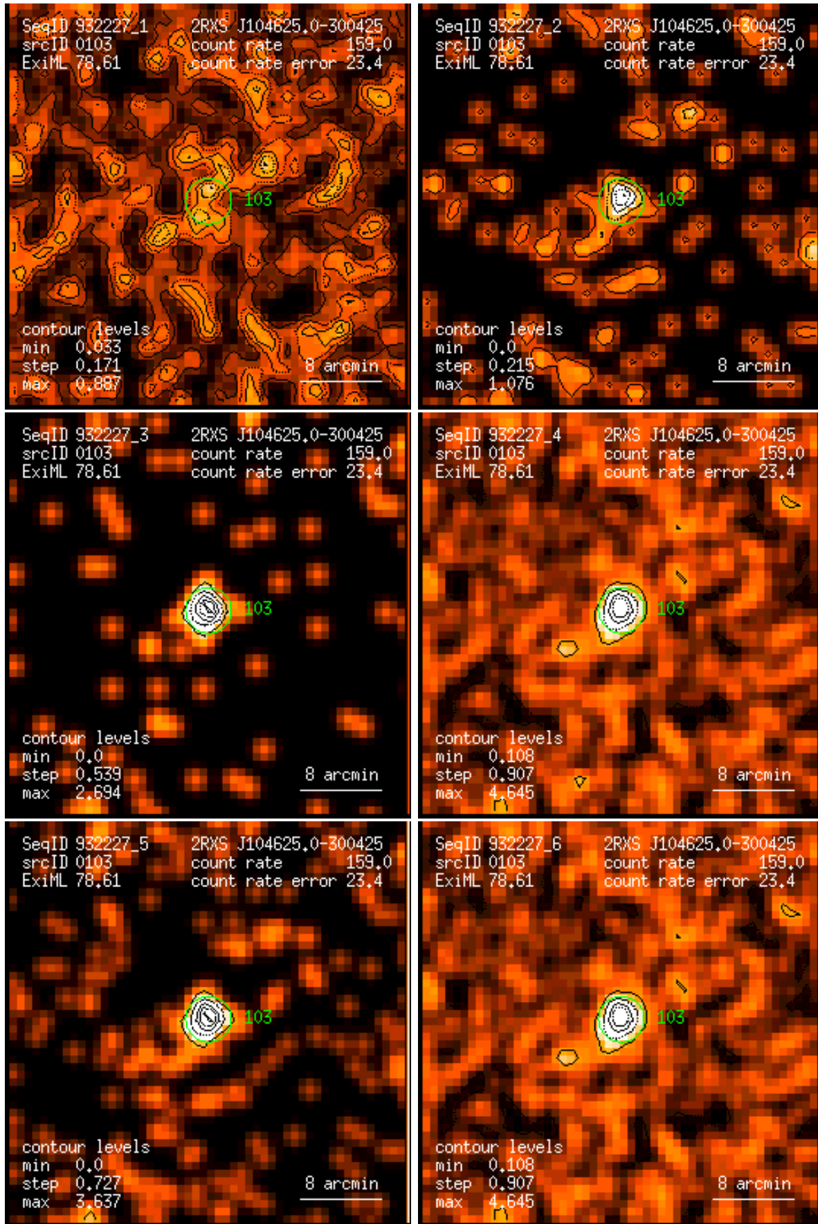
Figure 103: RASS 932227: detection 0103: band rate images, Gaussian filter: (1) PSPC channels 11 – 41, (2) 52 – 90, (3) 91 – 201, (4) 11 – 235, (5) 52 – 201, (6) 11 – 201. Broad band rates in counts/ks. Band rate contour levels in counts/ks/arcmin 2 .
