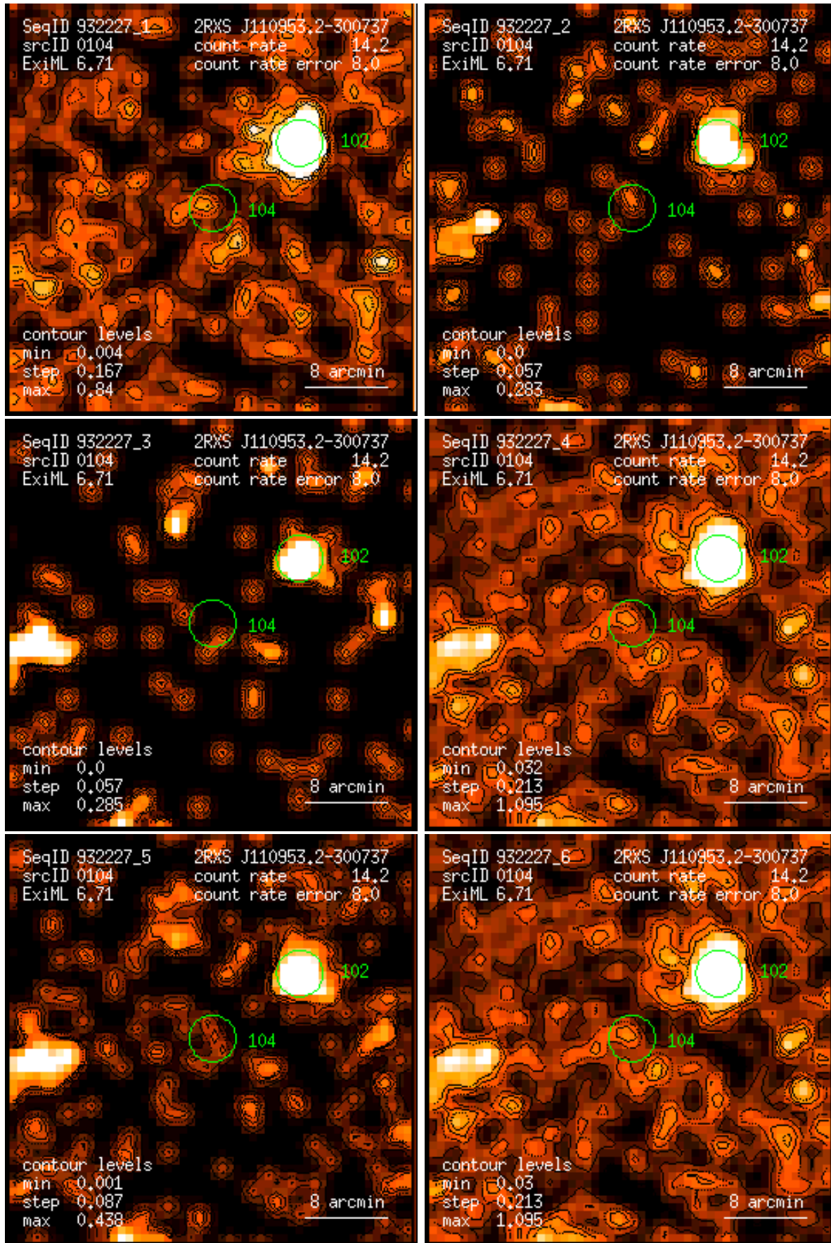
Figure 104: RASS 932227: detection 0104: band rate images, Gaussian filter: (1) PSPC channels 11 – 41, (2) 52 – 90, (3) 91 – 201, (4) 11 – 235, (5) 52 – 201, (6) 11 – 201. Broad band rates in counts/ks. Band rate contour levels in counts/ks/arcmin 2 .
