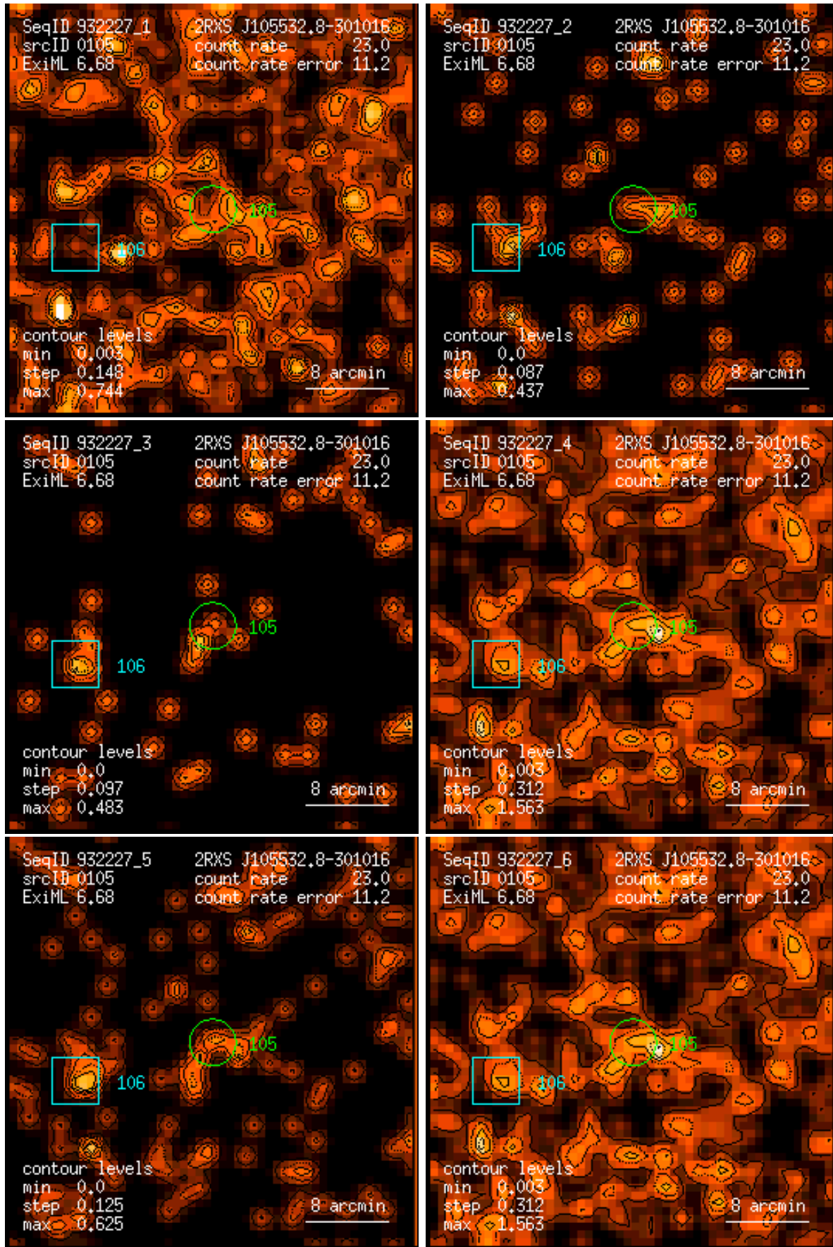
Figure 105: RASS 932227: detection 0105: band rate images, Gaussian filter: (1) PSPC channels 11 – 41, (2) 52 – 90, (3) 91 – 201, (4) 11 – 235, (5) 52 – 201, (6) 11 – 201. Broad band rates in counts/ks. Band rate contour levels in counts/ks/arcmin 2 .
