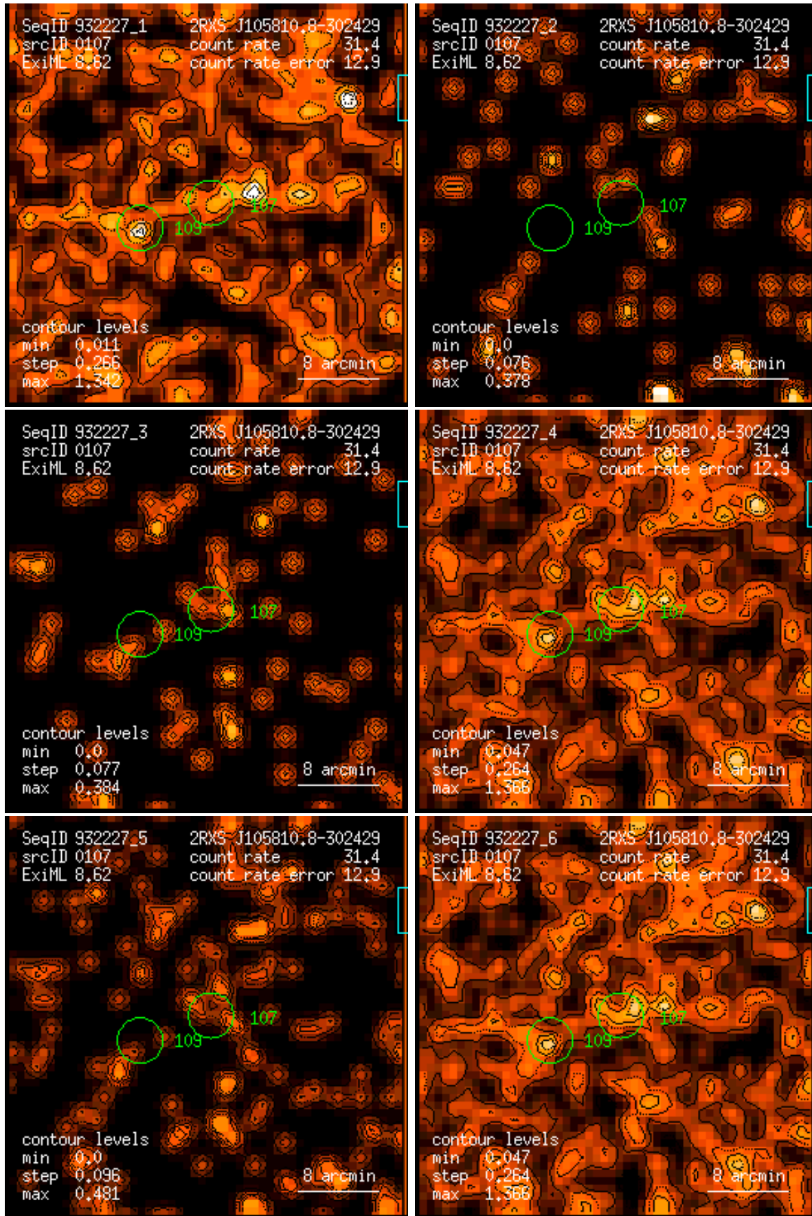
Figure 107: RASS 932227: detection 0107: band rate images, Gaussian filter: (1) PSPC channels 11 – 41, (2) 52 – 90, (3) 91 – 201, (4) 11 – 235, (5) 52 – 201, (6) 11 – 201. Broad band rates in counts/ks. Band rate contour levels in counts/ks/arcmin 2 .
