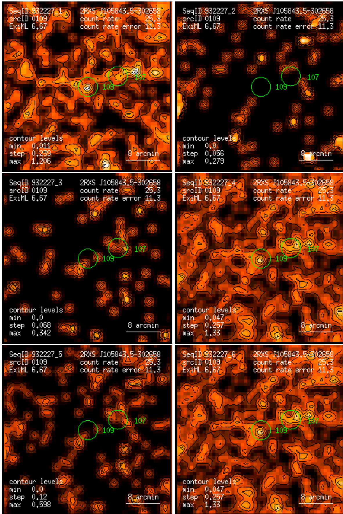
Figure 109: RASS 932227: detection 0109: band rate images, Gaussian filter: (1) PSPC channels 11 – 41, (2) 52 – 90, (3) 91 – 201, (4) 11 – 235, (5) 52 – 201, (6) 11 – 201. Broad band rates in counts/ks. Band rate contour levels in counts/ks/arcmin 2 .
