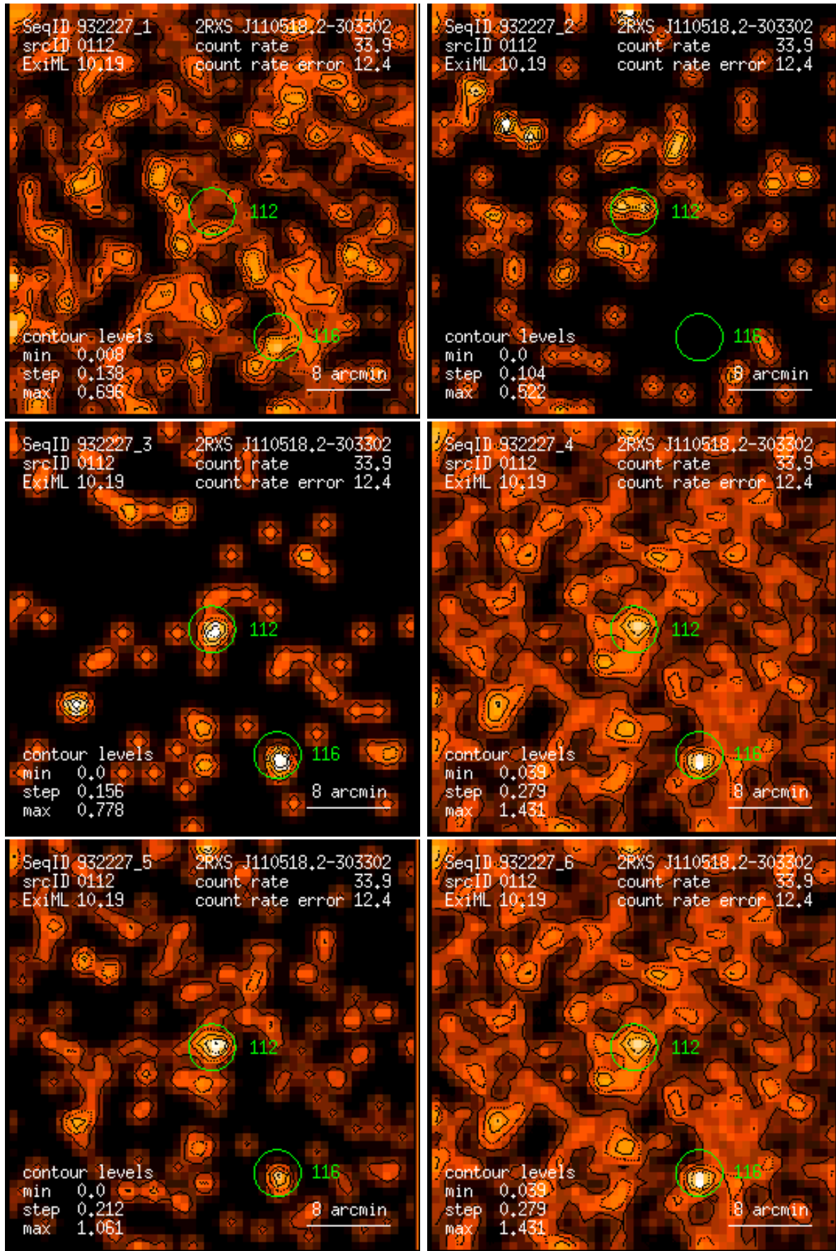
Figure 112: RASS 932227: detection 0112: band rate images, Gaussian filter: (1) PSPC channels 11 – 41, (2) 52 – 90, (3) 91 – 201, (4) 11 – 235, (5) 52 – 201, (6) 11 – 201. Broad band rates in counts/ks. Band rate contour levels in counts/ks/arcmin 2 .
