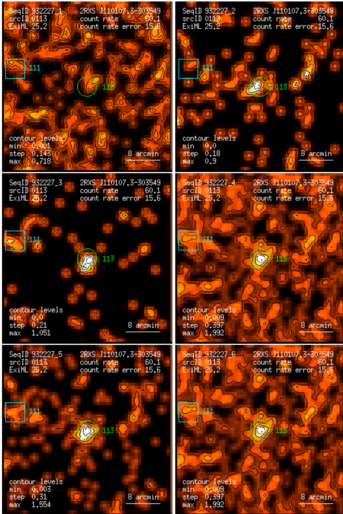
Figure 113: RASS 932227: detection 0113: band rate images, Gaussian filter: (1) PSPC channels 11 – 41, (2) 52 – 90, (3) 91 – 201, (4) 11 – 235, (5) 52 – 201, (6) 11 – 201. Broad band rates in counts/ks. Band rate contour levels in counts/ks/arcmin 2 .
