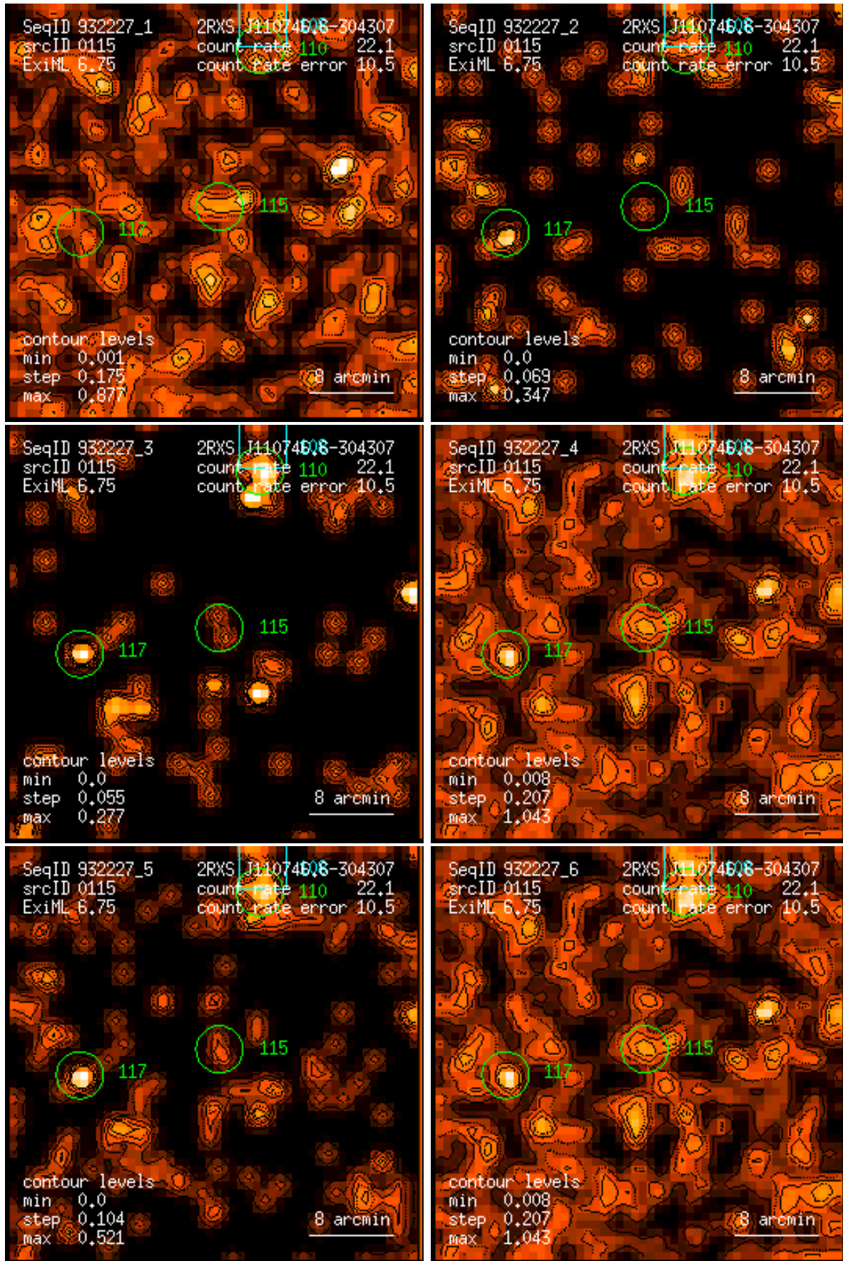
Figure 115: RASS 932227: detection 0115: band rate images, Gaussian filter: (1) PSPC channels 11 – 41, (2) 52 – 90, (3) 91 – 201, (4) 11 – 235, (5) 52 – 201, (6) 11 – 201. Broad band rates in counts/ks. Band rate contour levels in counts/ks/arcmin 2 .
